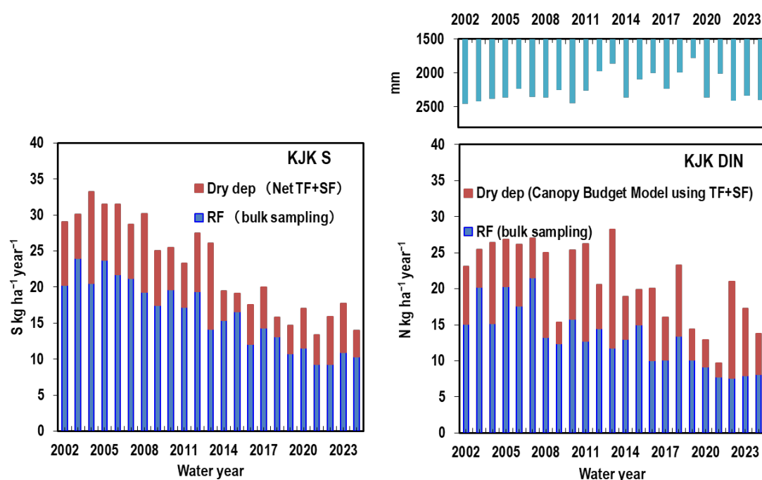
Fig. 1. Long-term changes in atmospheric sulfur (S) deposition and dissolved inorganic nitrogen (DIN) deposition. The water year is defined as June of one year through May of the following year. Dry deposition was estimated as the net throughfall and stemflow (TF + SF) for sulfur and using a canopy budget model (Staelens et al., 2008, Water, Air and Soil Pollution) for DIN. Modified from Sase et al. (2021).
