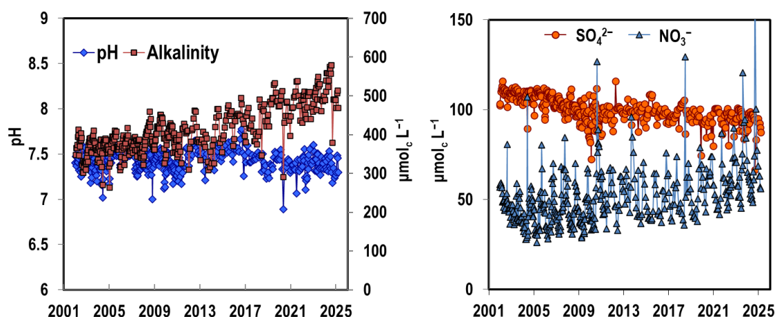
Fig. 2. Long-term changes in pH and alkalinity (left) and concentrations of \text{SO}_4^{2-} and \text{NO}_3^- (right).
