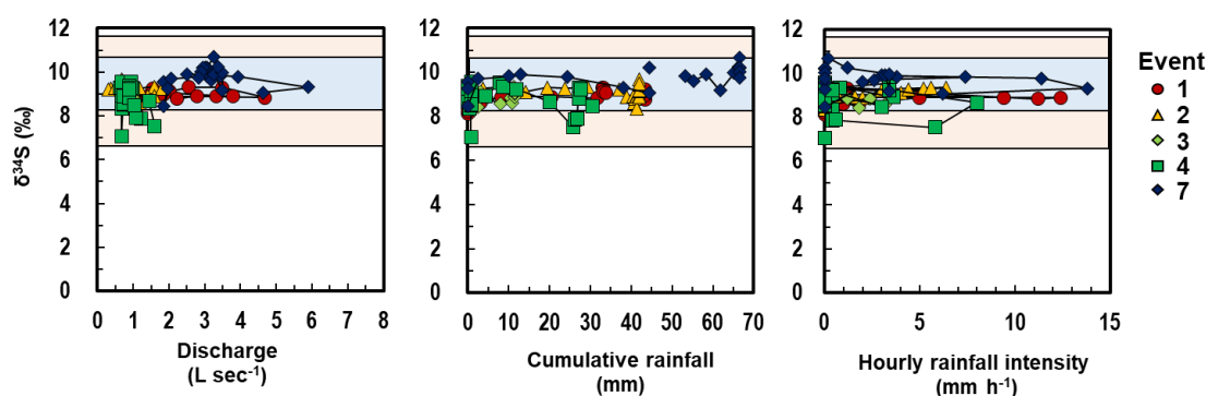
Fig. 4. Changes in \delta^{34}\text{S} values of stream water with (a) discharge, (b) cumulative rainfall, and (c) hourly rainfall intensity. The shaded area shows the range of \delta^{34}\text{S} values from August 2012 to November 2020 for stream water (SW: light blue) measured during the routine observations (Ministry of the Environment, 2019), and the range of the soil solution samples (SS: light orange) collected from 2012 to 2016 (Saito et al., 2023). Modified from Yotsuyanagi et al. (2024).
