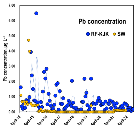
Fig. 5. Changes in monthly Pb concentration in rainwater (RF-KJK) and stream water (SW) at the Kajikawa catchment site. The dotted blue line shows a 3-month moving average. Modified from Morohashi et al. (2024).
