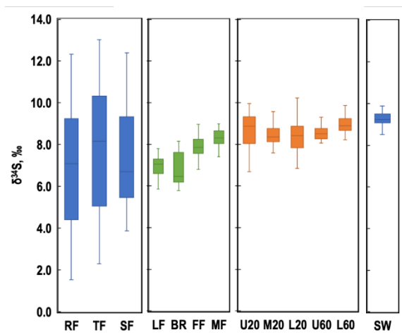
Fig. 3. Vertical changes in the sulfur isotopic ratio ( \delta^{34}\text{S} ) of rainfall outside forest canopy (RF), throughfall (TF), stemflow (SF), litterfall (leaf (LF), branch (BR), female flower (FF), and male flower (MF)), soil solutions (U20, M20, L20, U60, and L60), and stream water (SW) at the Kajikawa catchment (KJK). For soil solution, U, M, L indicate upper, middle, and lower slope positions, respectively and 20 and 60 indicate depths in cm. Modified from Saito et al. (2023).
