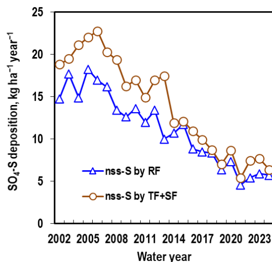
Fig. 6. Long-term changes in non-sea-salt (nss) sulfur deposition by rainfall outside forest canopy (RF) and throughfall and stemflow (TF + SF) at KJK. The water year is defined as June of one year through May of the following year. Modified from Sase et al. (2021).
