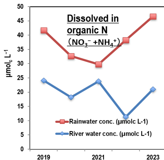
Figure 2.17. Comparison of Dissolved Inorganic Nitrogen Concentrations in Rainwater and Stream Water
