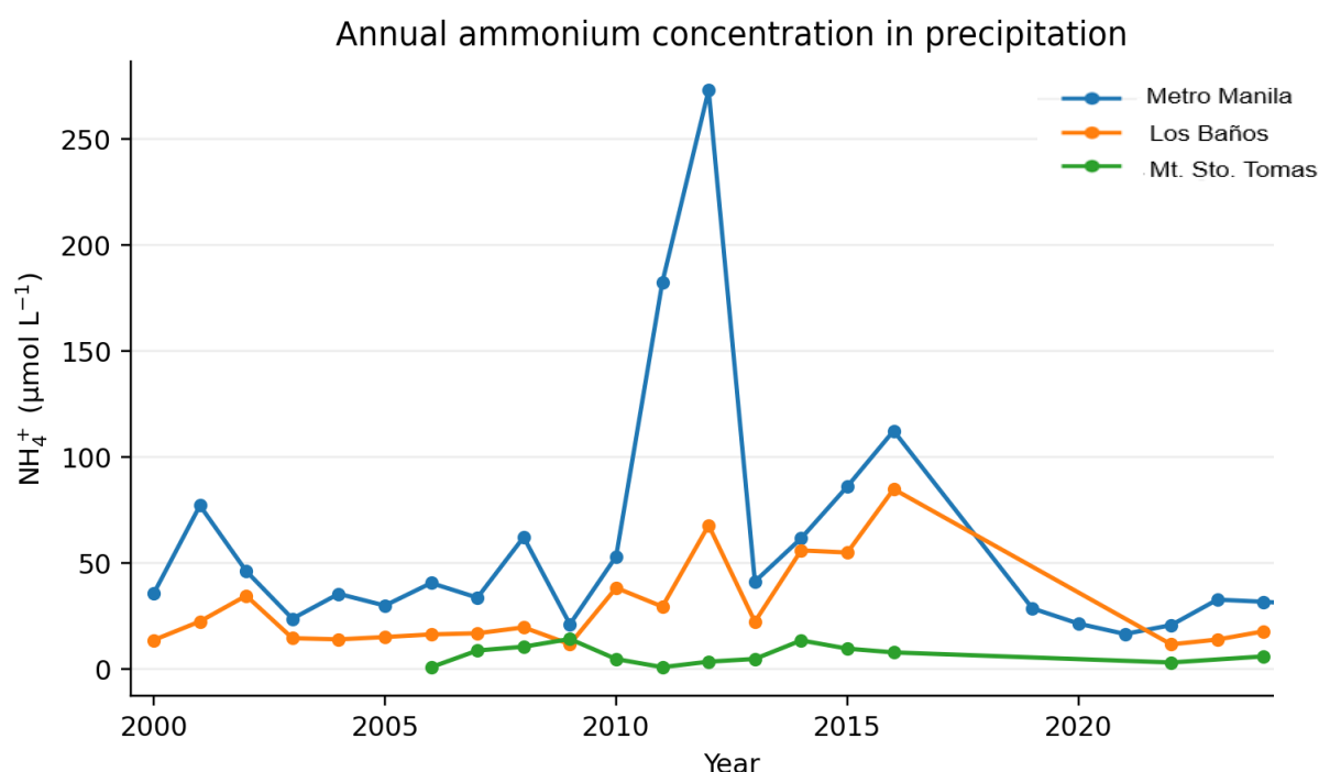
Figure 2.3. Annual ammonium concentrations at the three Philippine EANET monitoring sites for 2000–2024. The pronounced Metro Manila values in 2011–2012 are shown at their actual magnitudes.
