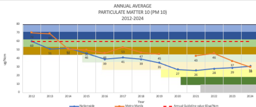
Figure 3.2. Particulate Matter 10 (PM 10) Annual Historical Data.
