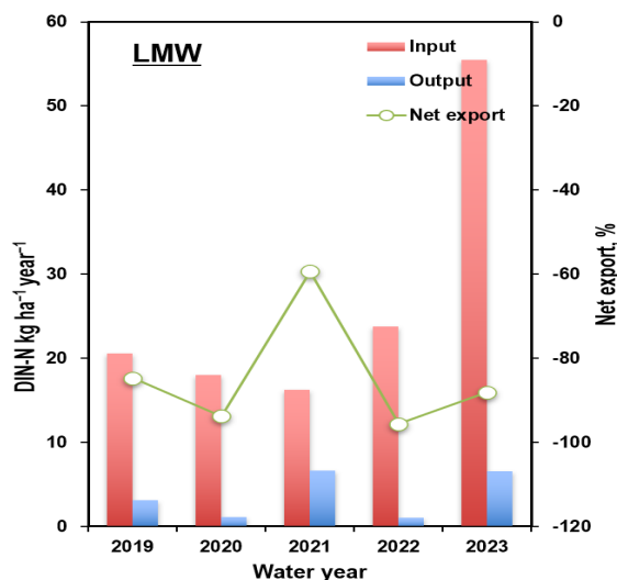
Figure 2.15. Dissolved Inorganic Nitrogen Input, Output, and Net Export
