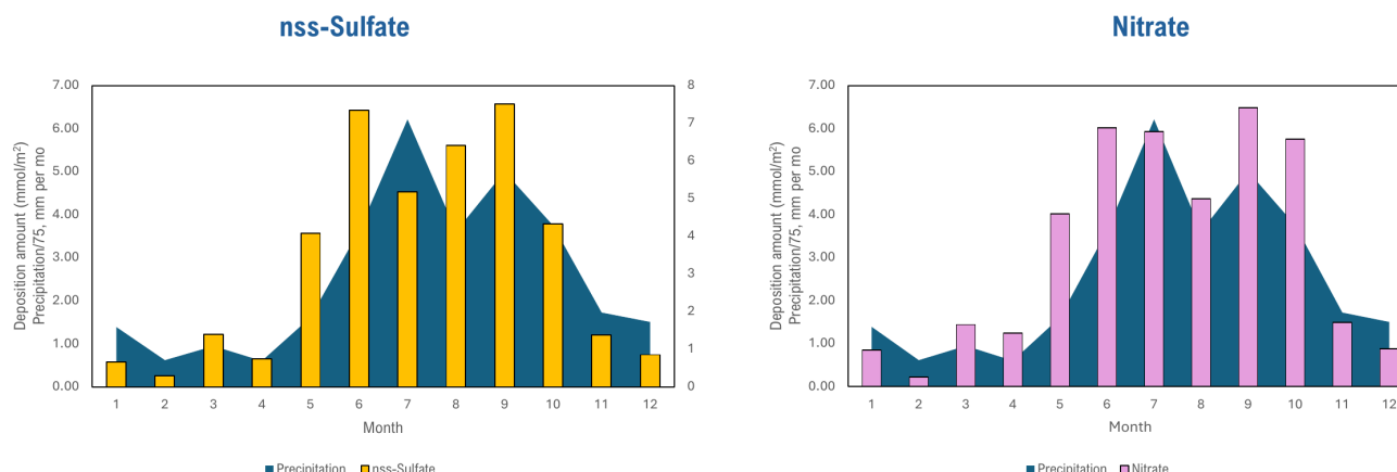
Figure 2.7. Supplied graphical representation of seasonal variation in Metro Manila nss-sulfate and nitrate deposition for 2019–2024, shown together with precipitation. Source: EANET STM 27 presentation.
