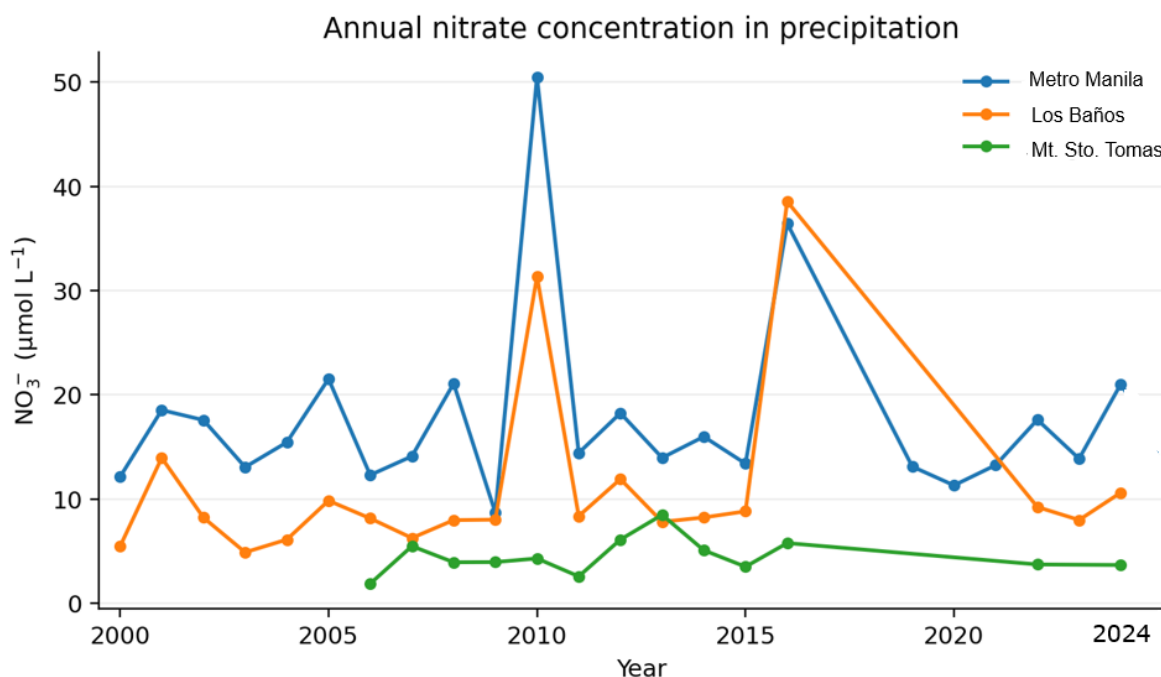
Figure 2.2 Annual nitrate concentrations at the three Philippine EANET monitoring sites from 2000 to 2024. Actual, unscaled concentrations are shown.
