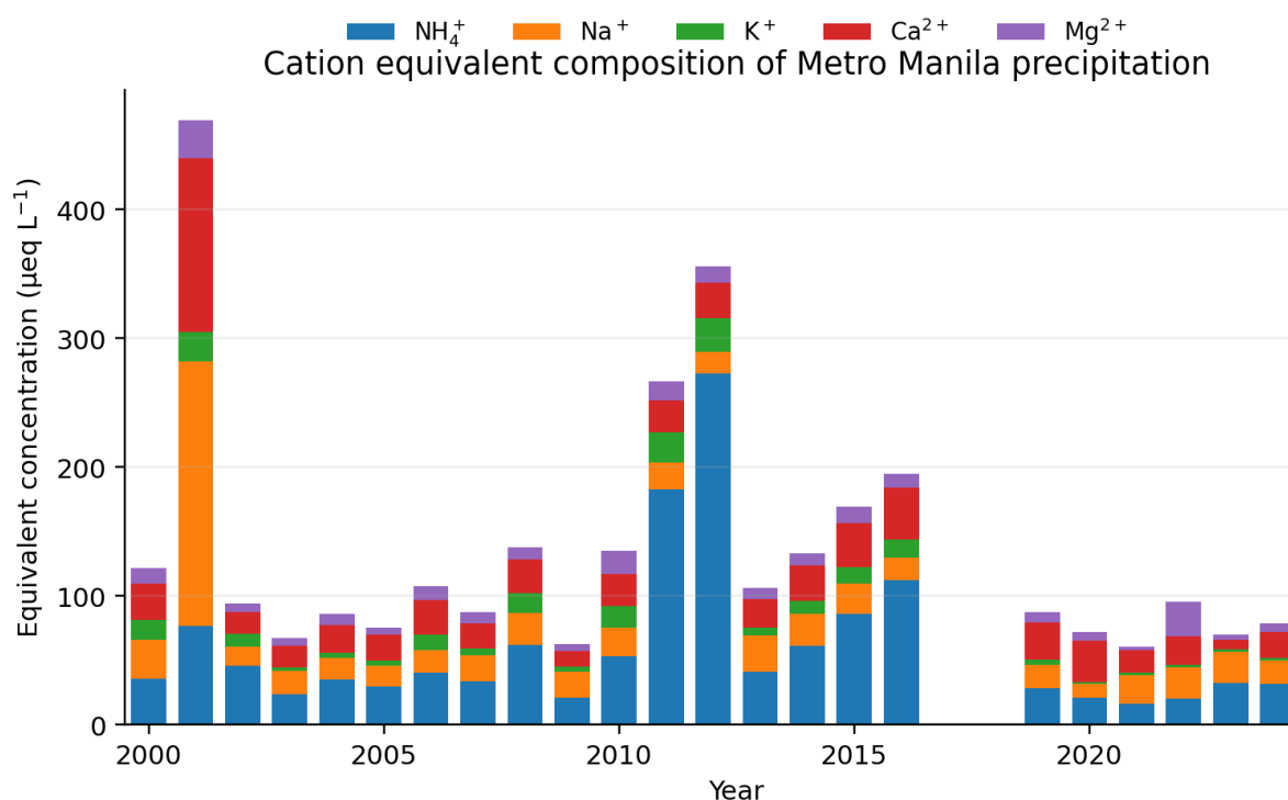
Figure 2.5. Cation equivalent composition of Metro Manila precipitation. Values are expressed as charge equivalents to support acid–base interpretation.
