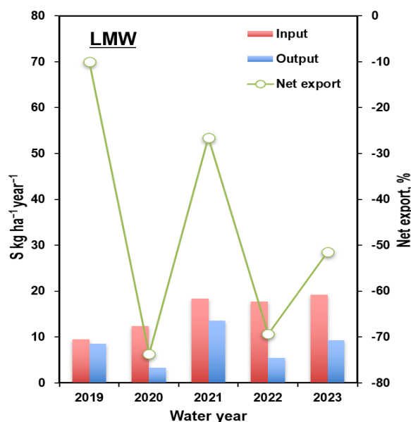
Figure 2.14. Sulfur Input, Output, and Net Export in LMW
