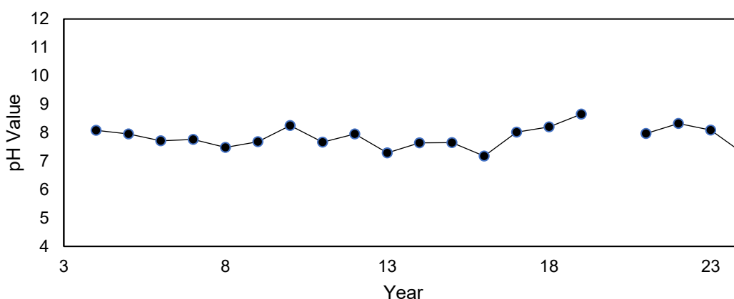
Figure 2.11. Long-term pH trends of of Lake Pandin from 2000 to 2024.
