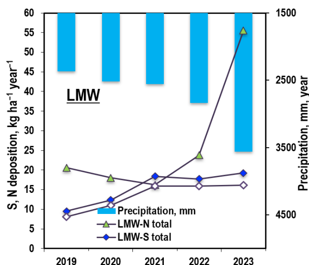
Figure 2.12. Annual Sulfur and Nitrogen Deposition in La Mesa Watershed (LMW) in relation to precipitation
