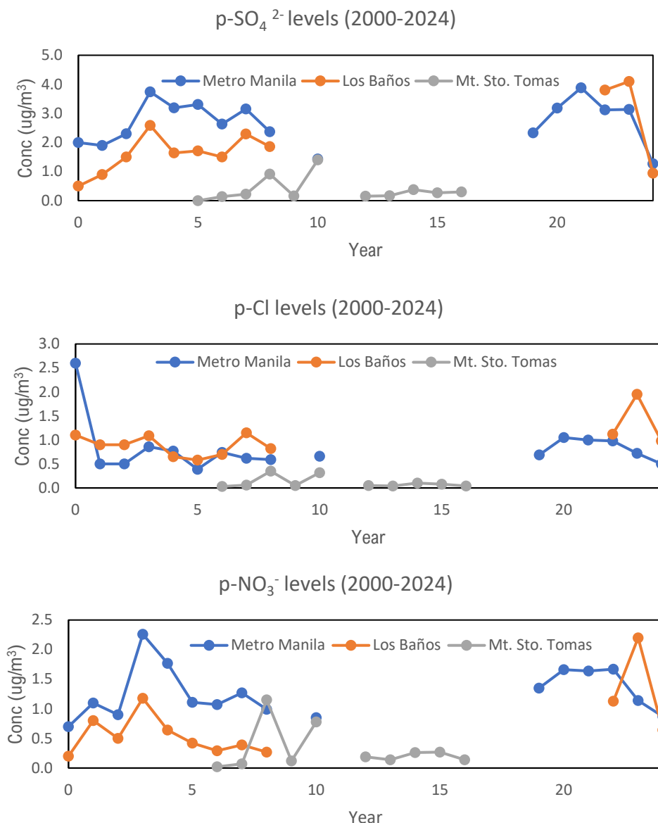
Figure 2.8. Annual Mean Concentration for particulate-bound sulfate, chloride, and nitrate for all monitoring sites from 2000 to 2024.
