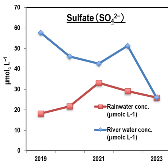
Figure 2.16. Comparison of Sulfate Concentrations in Rainwater and Stream Water
