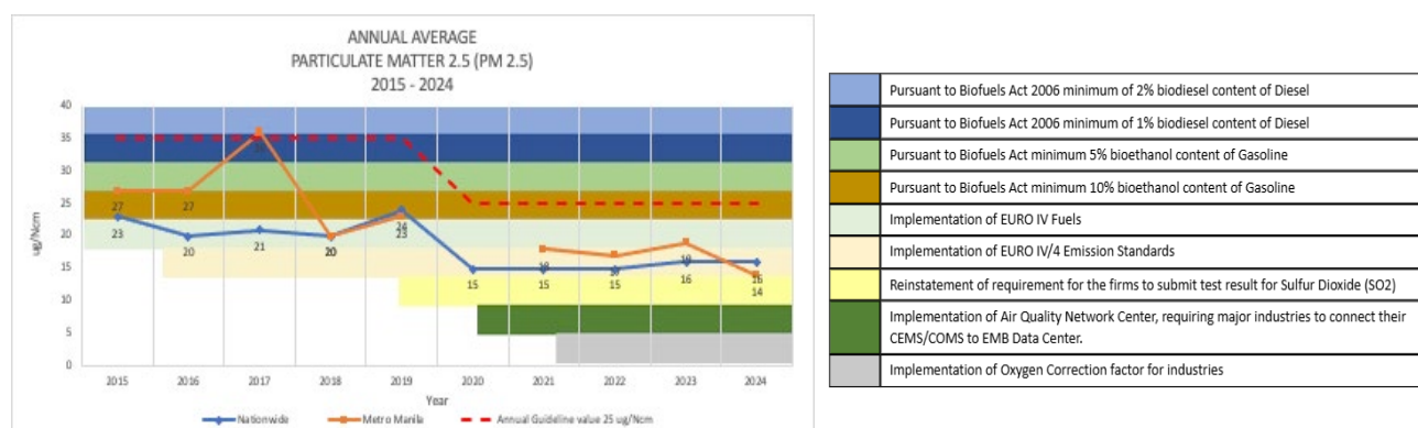
Figure 3.3. Particulate Matter 2.5 (PM 2.5) Annual Historical Data overlayed with years when policies relating to air quality management were implemented
