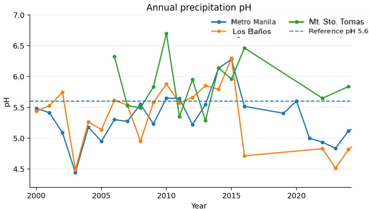
Figure 2.4. Annual precipitation pH at the three Philippine EANET monitoring sites from 2000 to 2024. The dashed line shows the pH 5.6 reference level used in the monitoring dataset.
