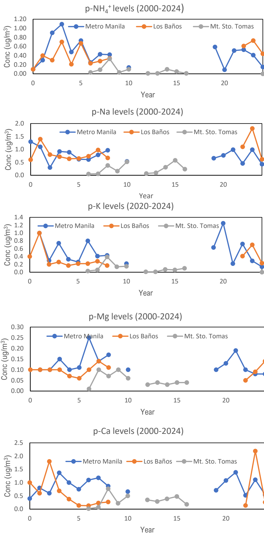
Figure 2.9. Annual Mean Concentration for particulate-bound cations for all monitoring sites from 2000 to 2024.
