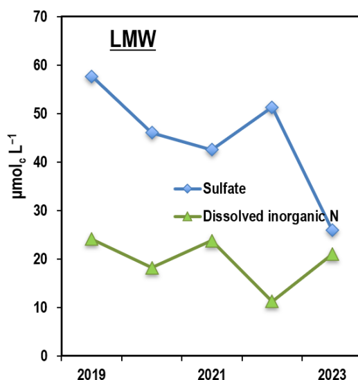
Figure 2.13. Annual Mean Sulfate and Dissolved Inorganic Nitrogen Concentrations in Stream Water
