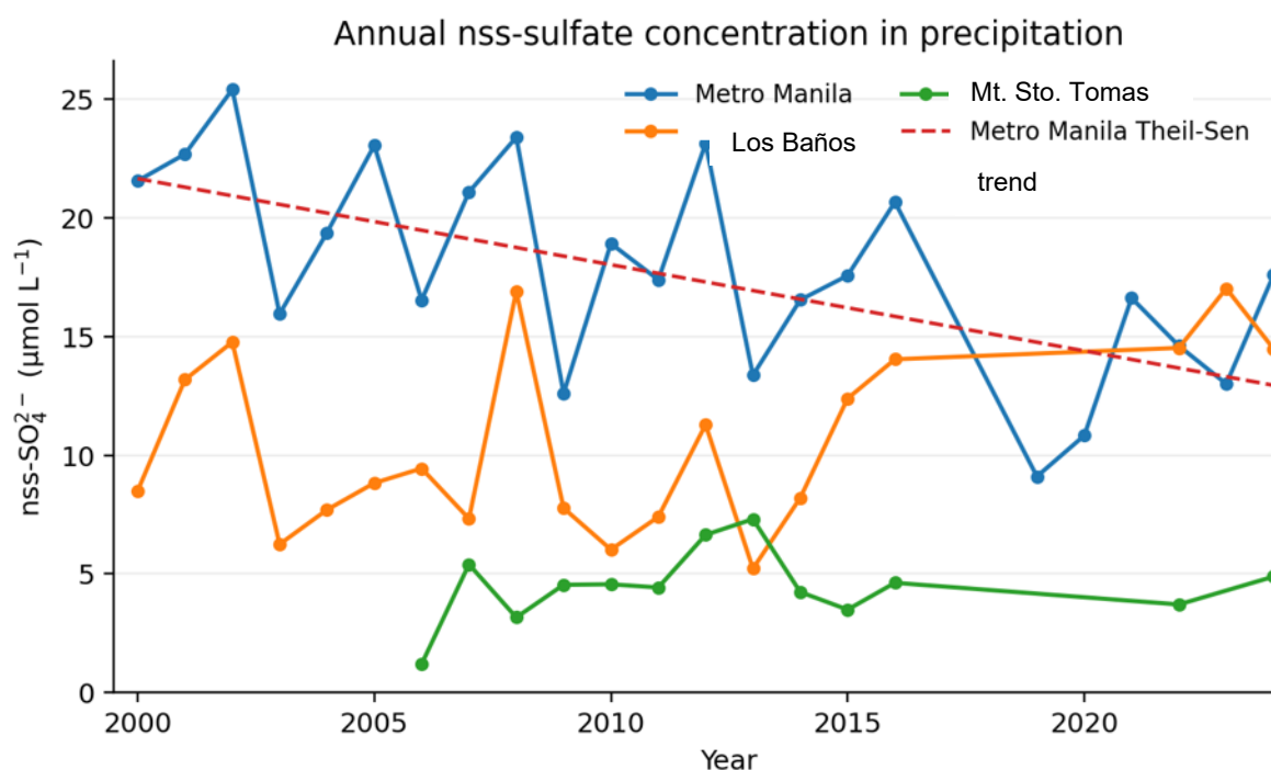
Figure 2.1. Annual nss-sulfate concentrations at the three Philippine EANET monitoring sites from 2000 to 2024. The dashed line represents the Theil–Sen trend for Metro Manila. Actual, unscaled concentrations are shown.
