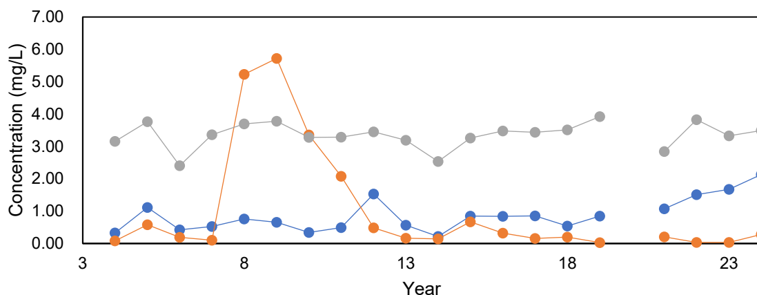
Figure 2.10. Long-term trends of sulfate, nitrate, and chloride from 2000 to 2024 from Lake Pandin.
