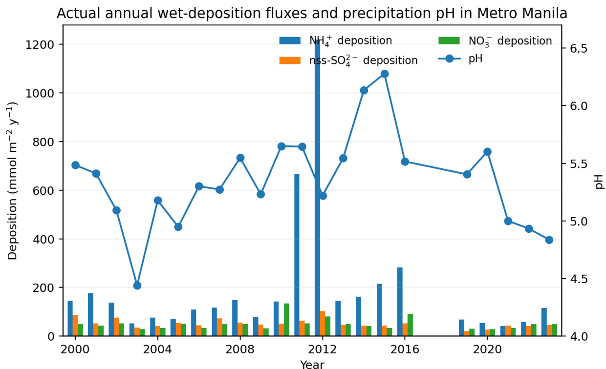
Figure 2.6. Actual annual ammonium, nss-sulfate, and nitrate wet-deposition fluxes in Metro Manila with annual precipitation pH. Fluxes were recalculated from unscaled concentration and precipitation data.
