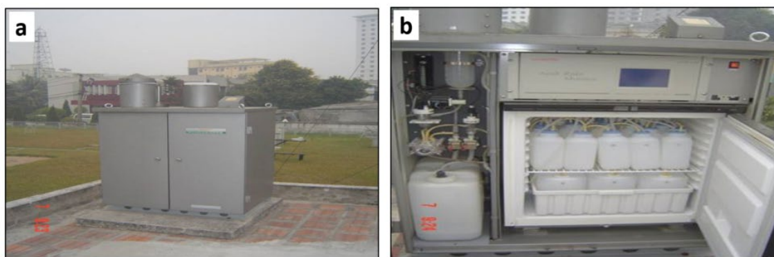
Figure 1. Wet Sampler (Kimoto MCSAM-6-VB).
