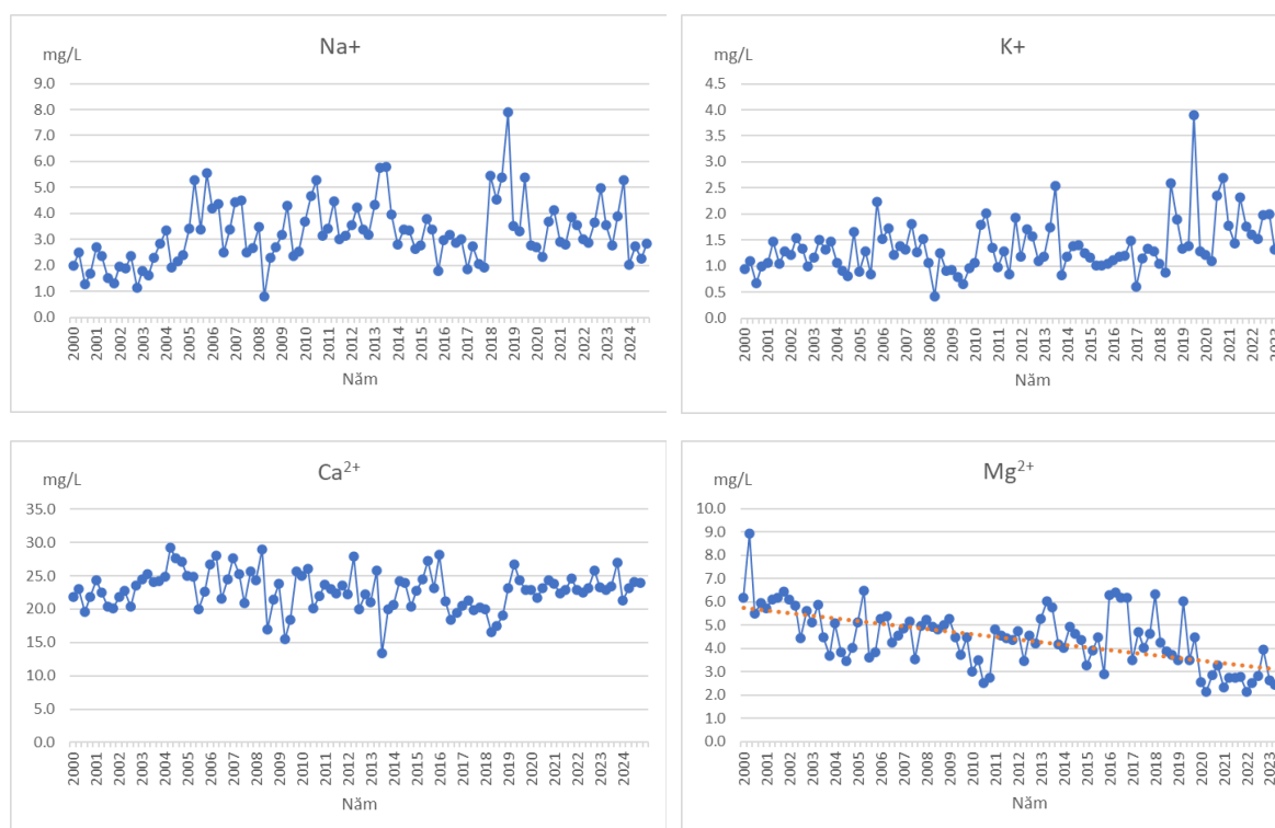
Fig 321. Temporal variation of water chemistry in Hoa Binh Reservoir (2000- 2024)
