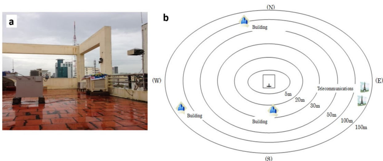
Figure 10. (a) Picture of Ho Chi Minh station and (b) Profile of Ho Chi Minh station on-site scale (150m).
