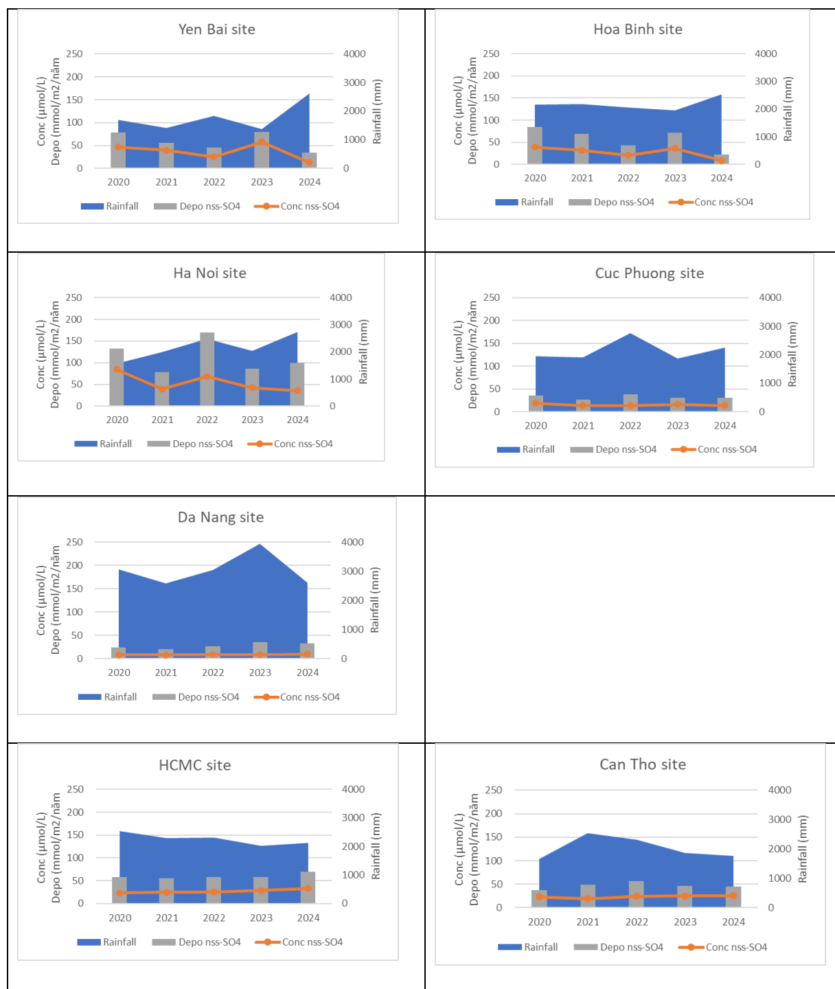
Fig.16. Relationship between nss-SO_4^{2-} Concentrations, Precipitation Amount, and Wet Deposition Flux
