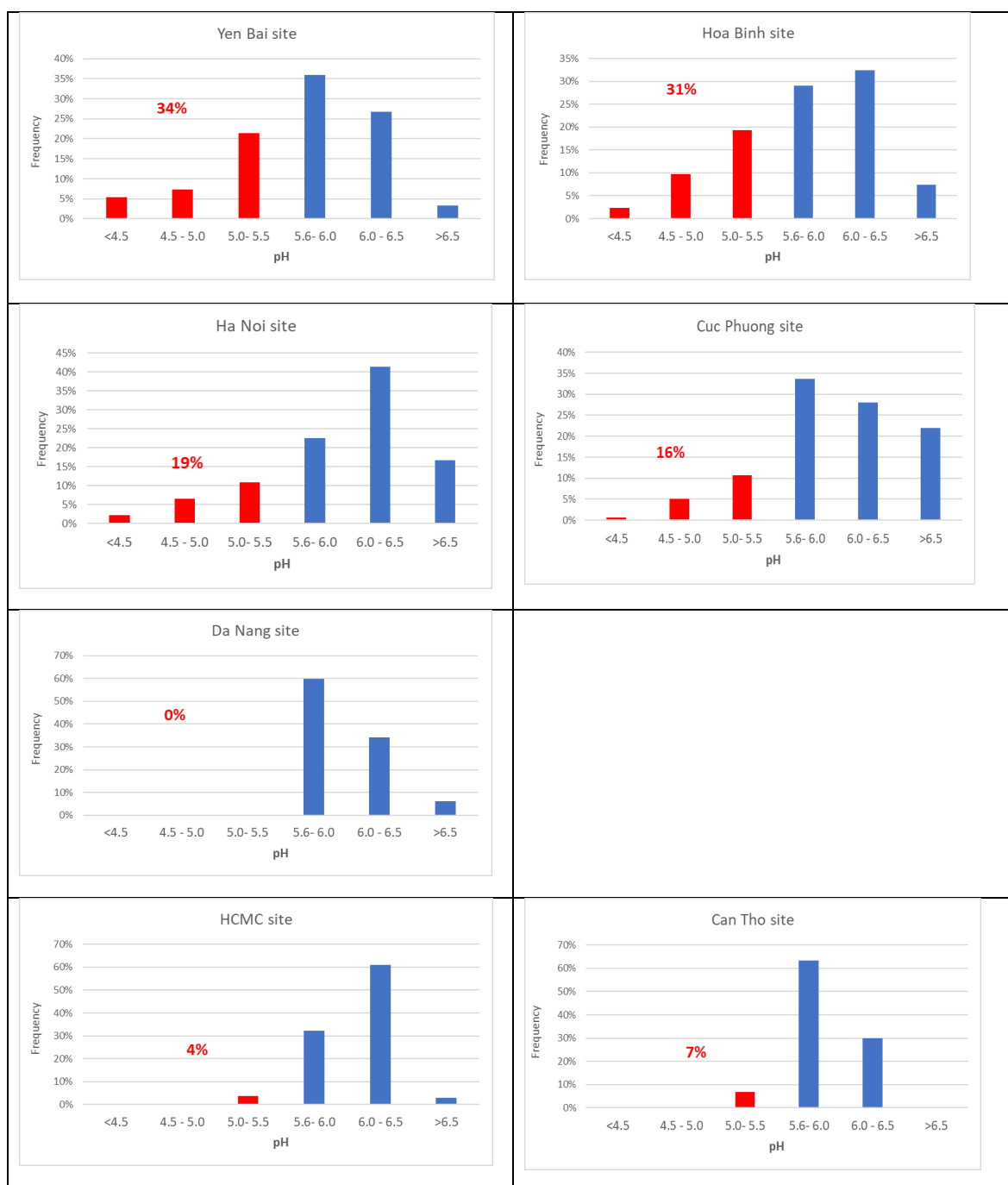
Figure 14. Frequency of acid rain (pH < 5.6) in sites (2020 – 2024)
