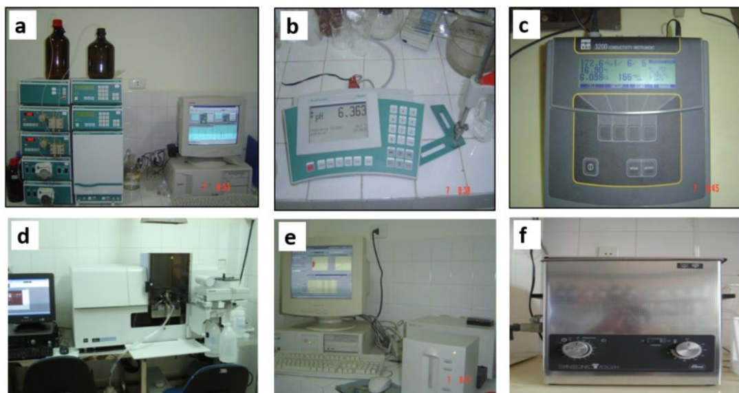
Figure 2. Equipment for Acid Deposition Analysis (a) IC Metrohm Mic 3, (b) pH meter – 793, (c) EC meter – YSI 3200, (d) AAS800 of PerkinElmer, (e) UV-Vis – HP8453 and (f) Ultrasonic bath.
