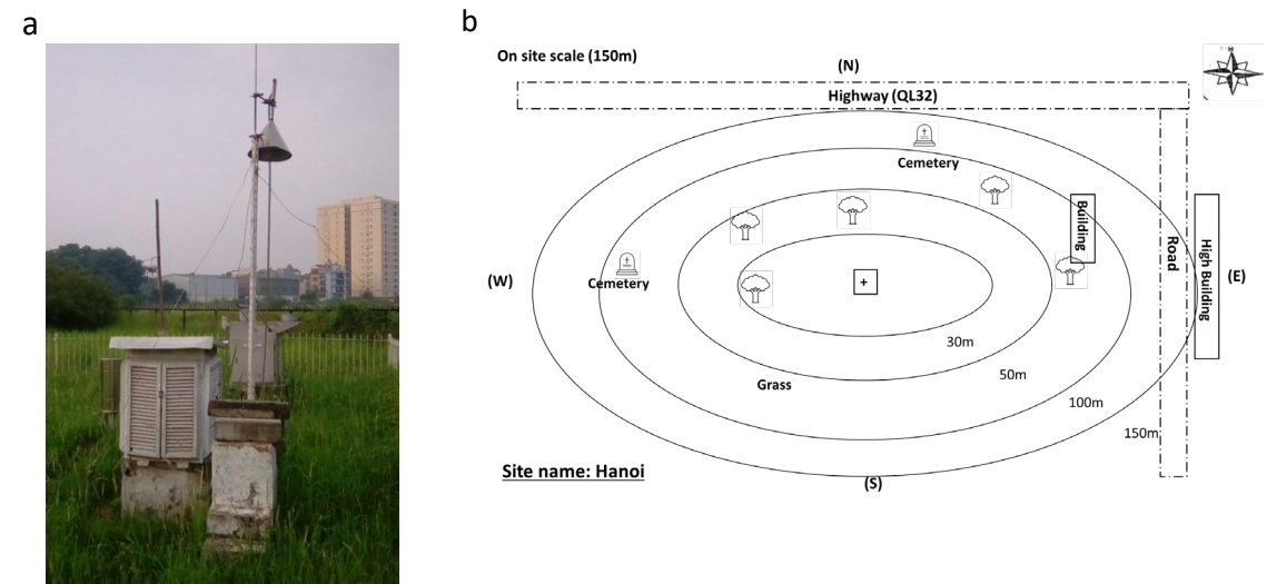
Figure 5. (a) Picture of Ha Noi station and (b) Profile of Hanoi station: on-site scale (150m).
