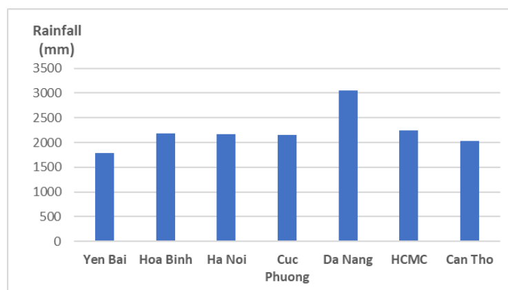
Fig 15. Annual rainfall amount in sites (2020-2024)
