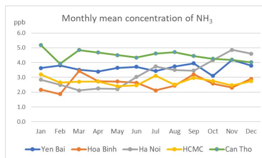
Fig.30. Monthly variation of NH 3 concentrations at Sites
