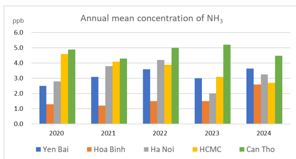
Fig.29. Temporal variation of NH 3 concentrations at Sites (2020- 2024)
