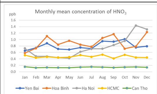
Fig.26. Monthly variation of HNO 3 concentrations at Sites
