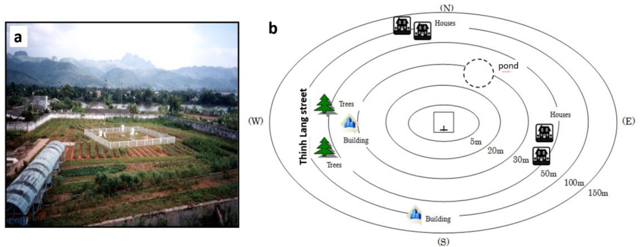
Figure 6. (a) Picture of Hoa Binh station and (b) Profile of Hoa Binh station: on-site scale (150m).
