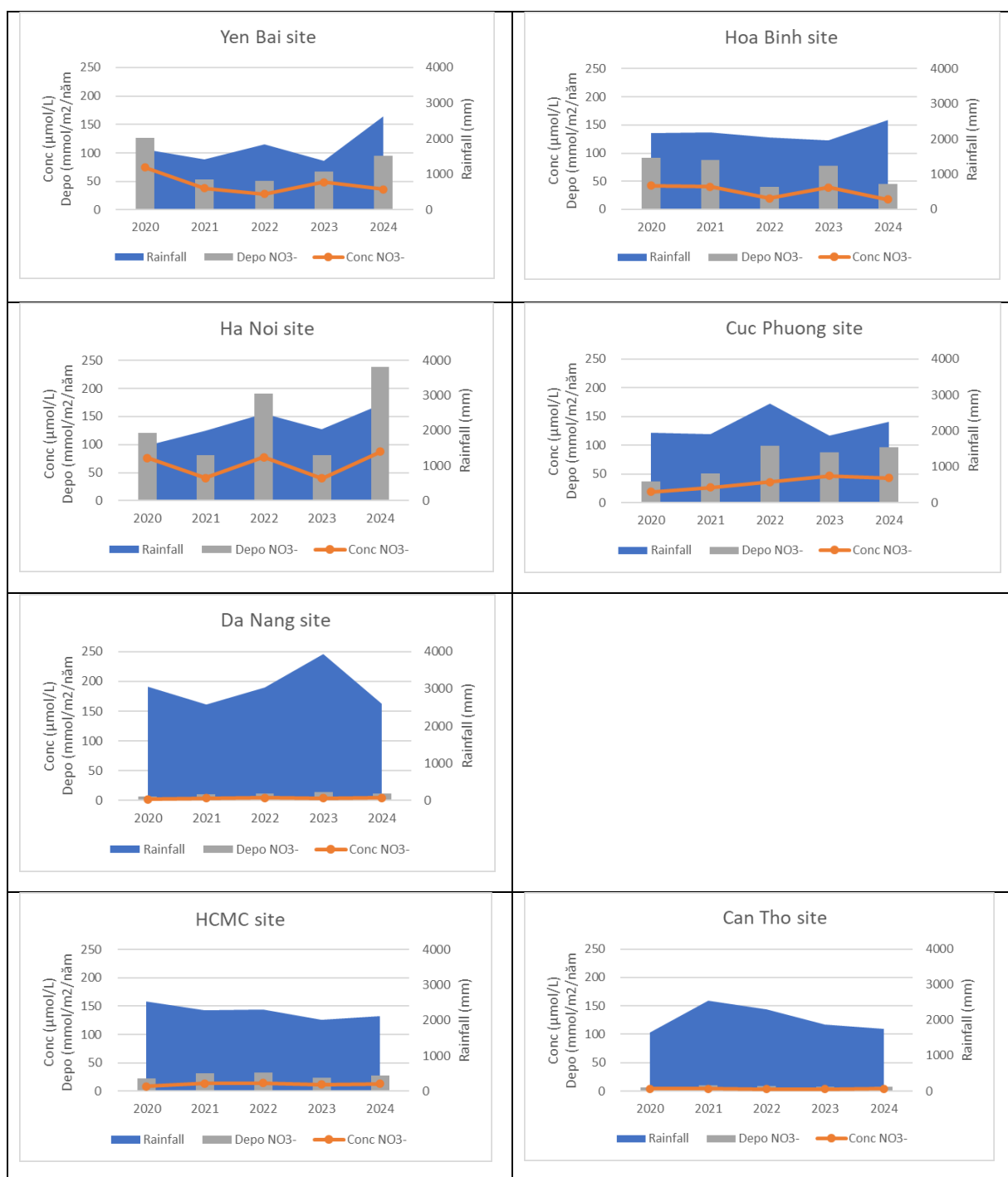
Fig. 17. Relationship between \text{NO}_3^- concentrations, Precipitation Amount, and Wet Deposition Flux
