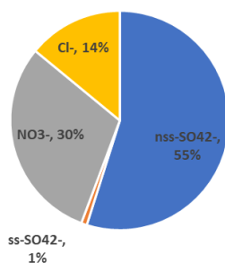
Anion composition in Hoa Binh
