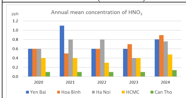
Fig.25. Temporal variation of HNO 3 concentrations at Sites (2020-2024)
