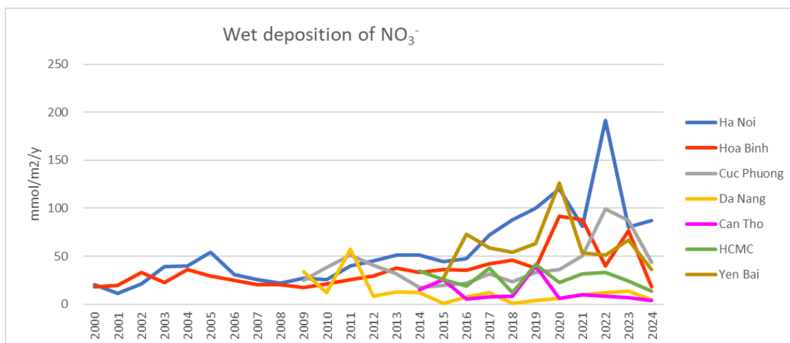
Fig. 21. Temporal variation of \text{NO}_3^- Wet deposition (2000–2024)
