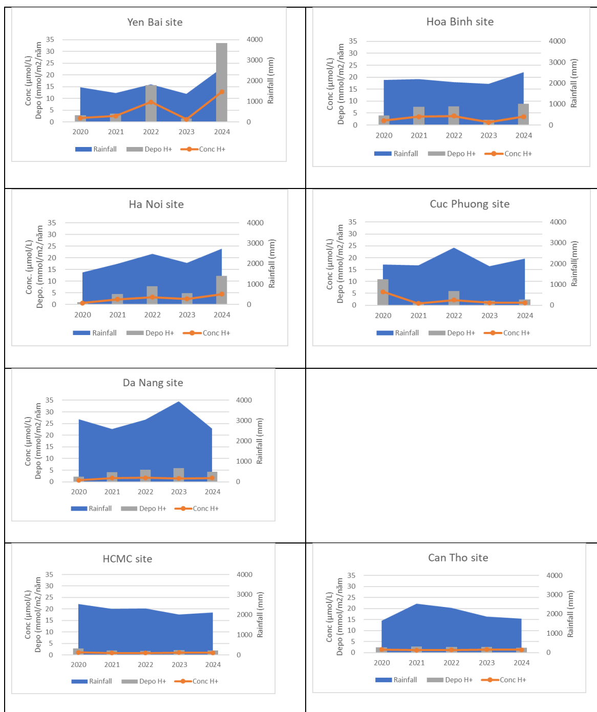
Fig. 18. Relationship between H^+ Concentrations, Precipitation Amount, and Wet Deposition Flux
