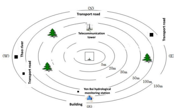
Figure 4. (a) Picture of Yen Bai station and (b) Profile of Yen Bai station: on-site scale (150m).
