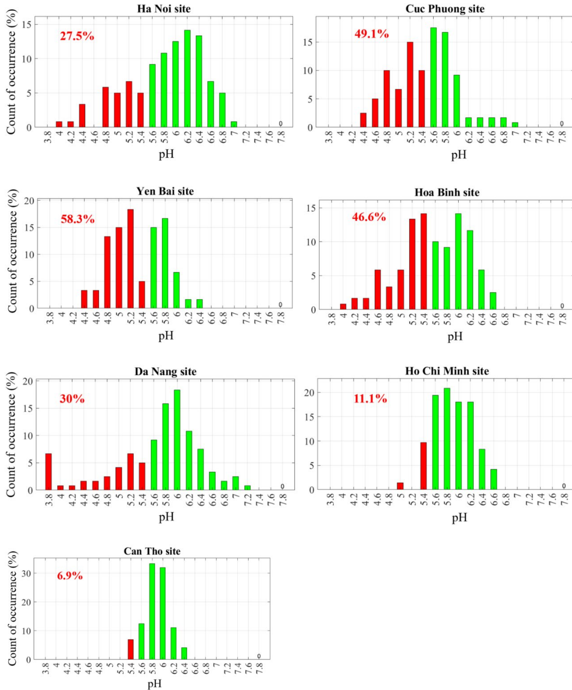
Figure 13. Frequency of acid rain (pH < 5.6) in sites (2015 – 2019)
