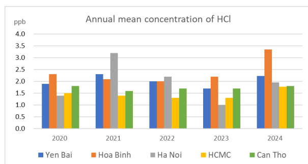
Fig.27. Temporal variation of HCl concentrations at Sites (2020- 2024)
