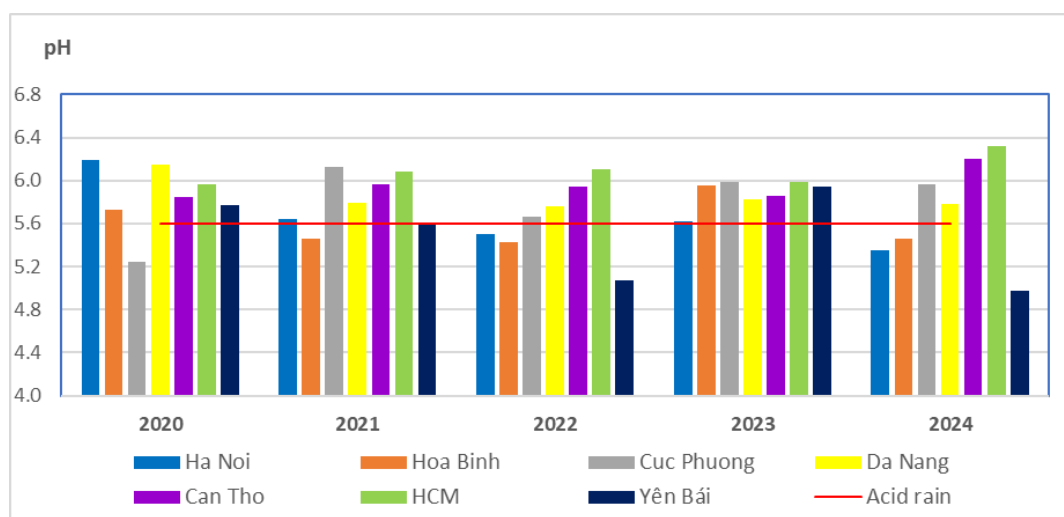
Figure 11. Annual mean pH of rainwater in sites (2020 – 2024)
