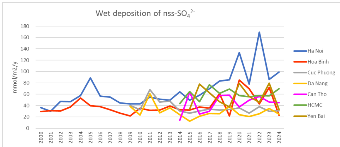
Fig. 20. Temporal variation of \text{nss-SO}_4^{2-} Wet deposition (2000–2024)
