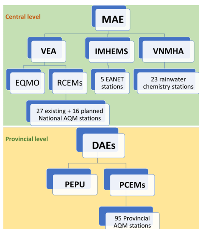
Fig. 33. Institutional structure of Air quality management system including Acid deposition in Vietnam
