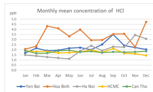
Fig.28. Monthly variation of HCl concentrations at Sites
