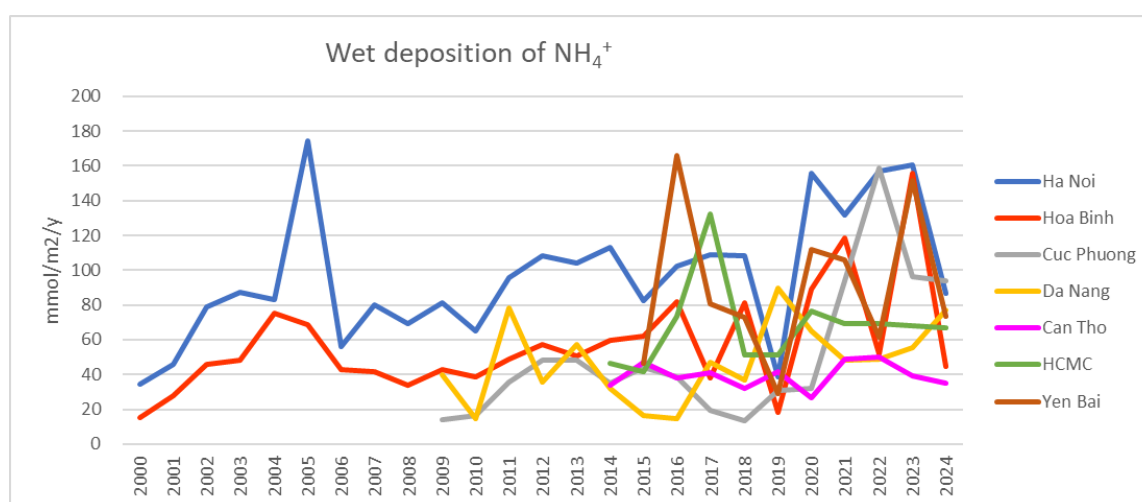
Fig. 22. Temporal variation of \text{NH}_4^+ Wet deposition (2000–2024)
