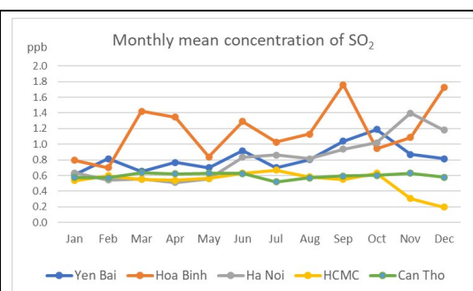
Fig. 24. Monthly variation of SO 2 concentrations at Sites
