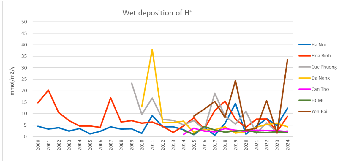
Fig. 19. Temporal Variation of \text{H}^+ Wet Deposition (2000–2024)
