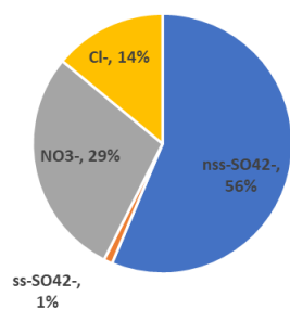
Anion composition in Ha Noi
