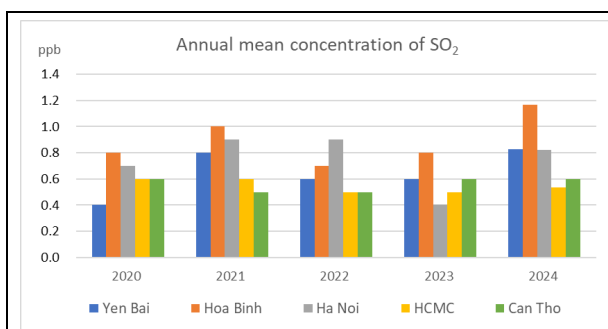
Fig.23. Temporal variation of SO 2 concentrations at Sites (2020-2024)
