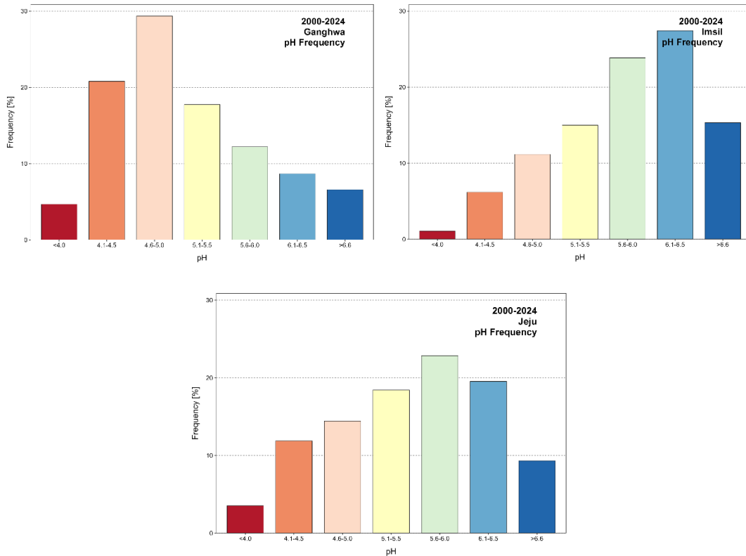
Figure 1.2.5. pH frequency and the amount in each site (2000~2024).
