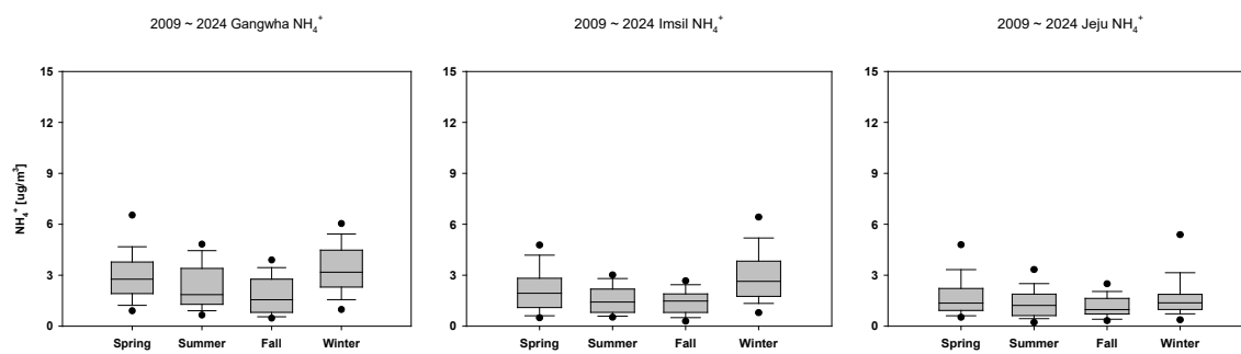
Figure 1.2.14. Seasonal variations of major chemical species concentrations in \text{PM}_{2.5} at sites.
