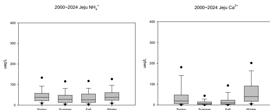
Figure 1.2.9. Seasonal variation of wet deposition (equivalent concentration), Jeju.
