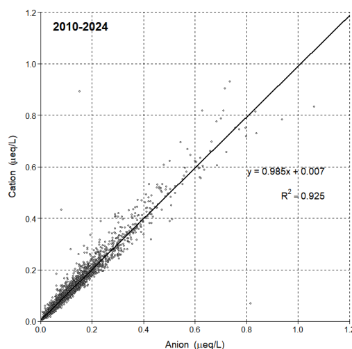
Figure 1.2.10. Relationship between total anion and cation.
