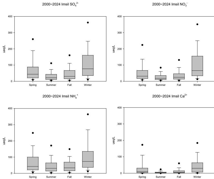
Figure 1.2.8. Seasonal variation of wet deposition (equivalent concentration), Imsil.
