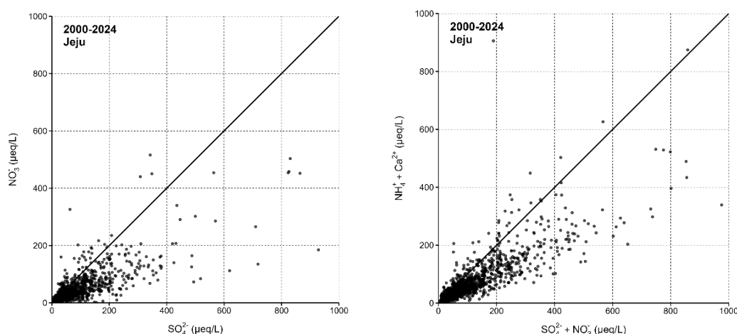
Figure 1.2.3. Ion balance check in Ganghwa, Imsil and Jeju (Unit: µeq/L).
