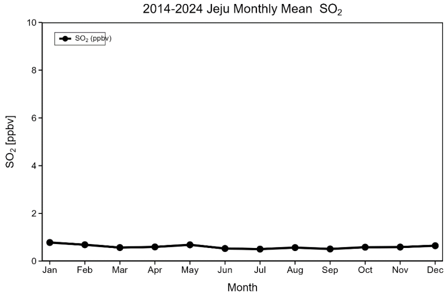
Figure 1.2.13. Average monthly concentrations of SO 2 , NO 2 , O 3 and PM 10 at Jeju.
