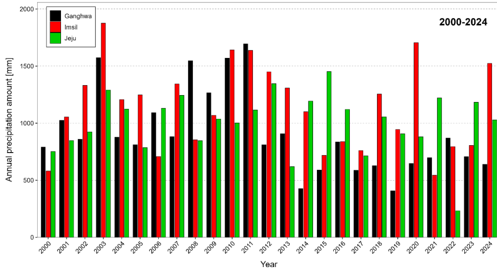
Figure 1.2.4. The annual average pH and precipitation amount at each site (2000~2024).
