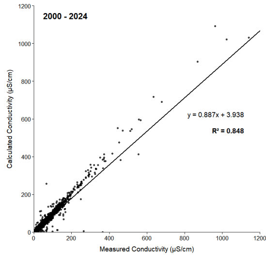
Figure 1.2.2. Relationship between the \text{EC}_{\text{meas}} and \text{EC}_{\text{cal}} .
