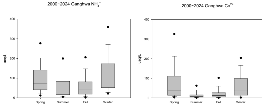
Figure 1.2.7. Seasonal variation of wet deposition (equivalent concentration), Ganghwa
