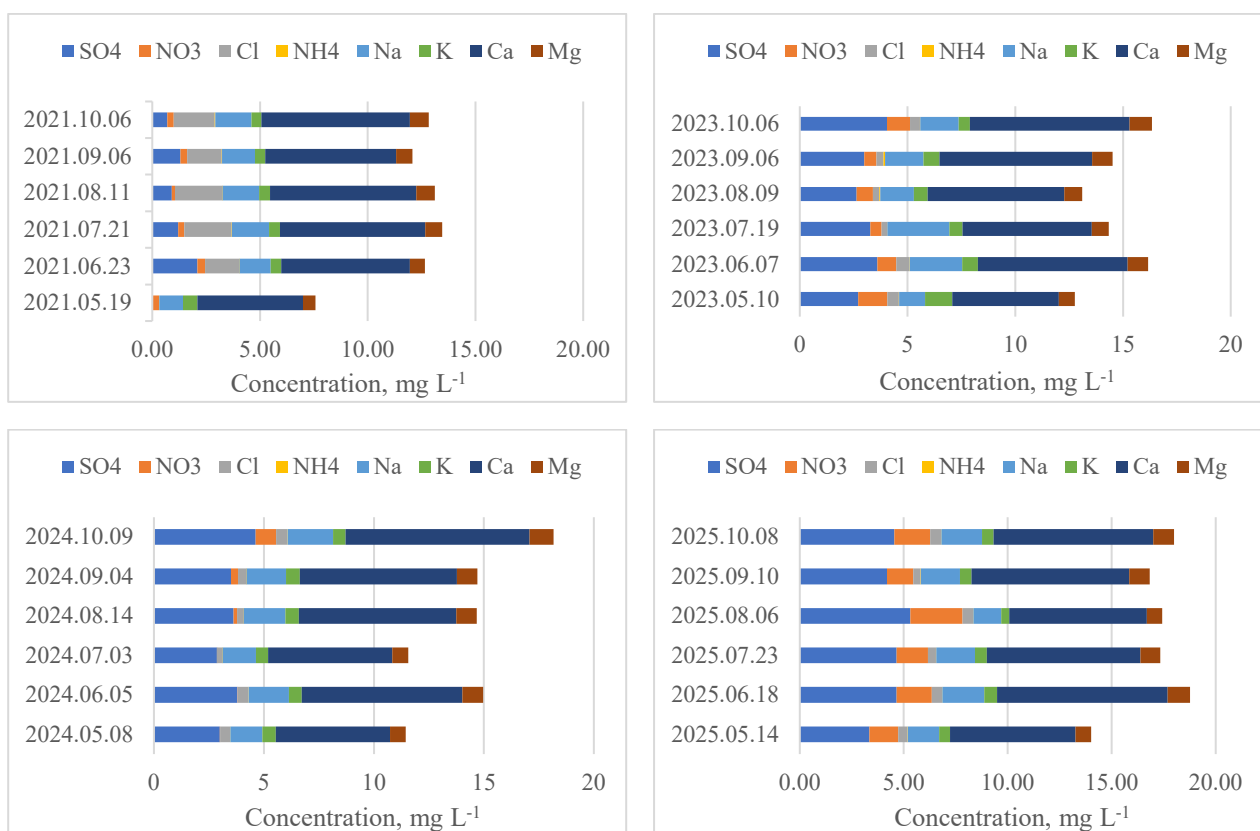
Figure 19. Major-ion concentrations in the Terelj River in 2021 and 2023–2025; complete ion measurements were unavailable for 2022.
