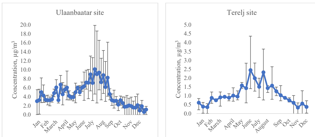
Figure 8. Ammonia concentration at sampling sites. Error bars indicate the minimum and maximum measured concentrations during the monitoring period.
