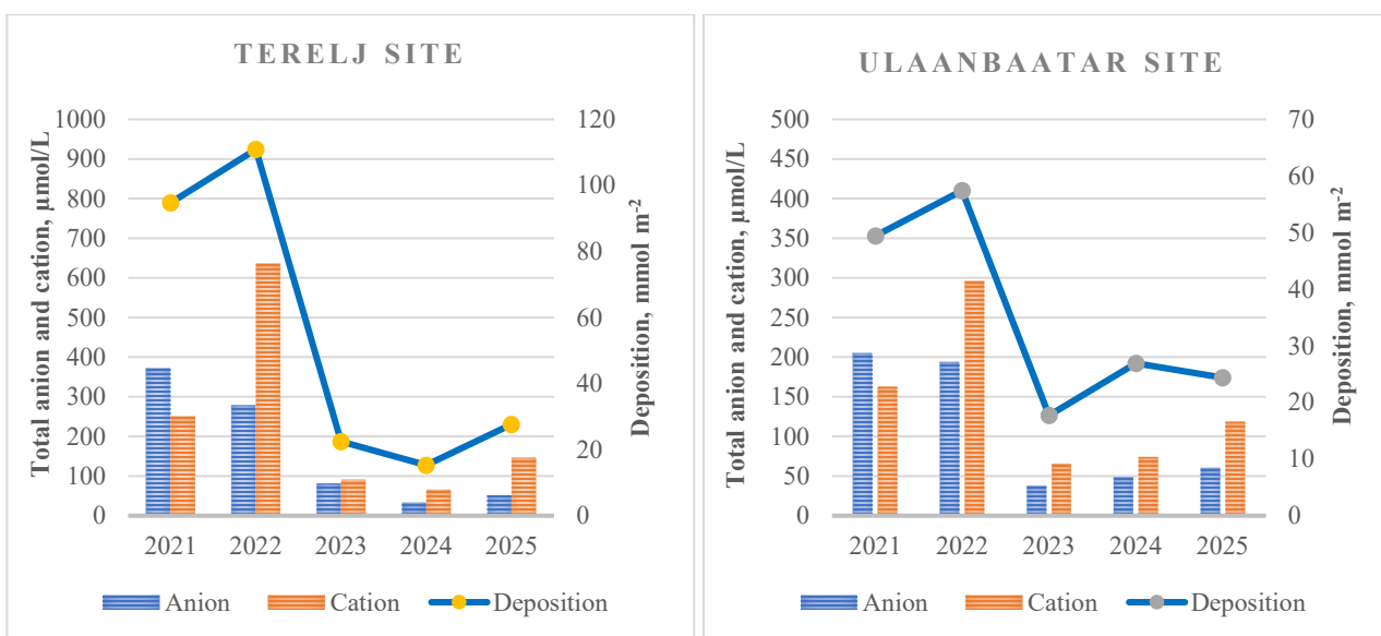
Figure 15. Interannual variation in total anion and cation concentrations and wet-deposition flux at Terelj and Ulaanbaatar during the May–October monitoring periods, 2021–2025.
