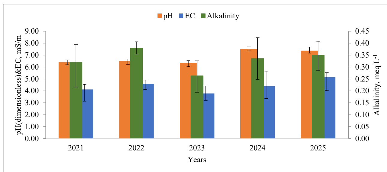
Figure 18. Interannual variability in pH, electrical conductivity (EC), and alkalinity. Error bars indicate the minimum and maximum measured values within each monitoring year.
