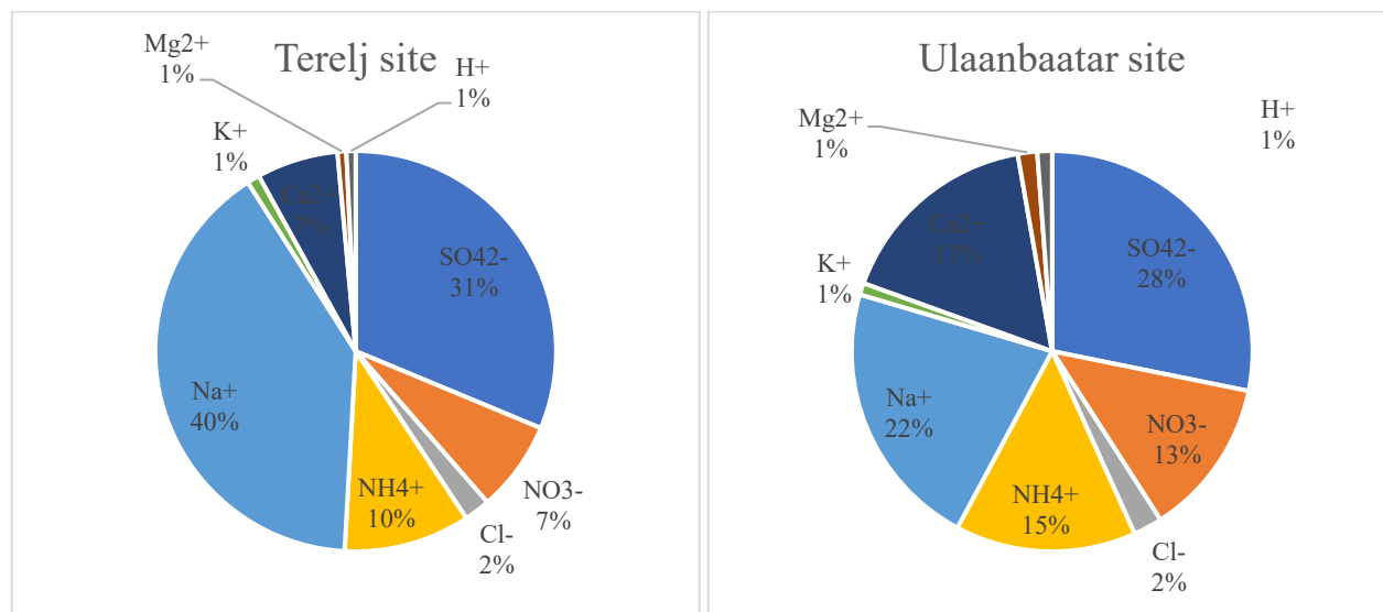
Figure 14. Relative composition of major ions in wet-deposition samples collected during May–October at Terelj and Ulaanbaatar, 2021–2025, calculated from mean ion concentrations expressed in \mu\text{mol L}^{-1} .
