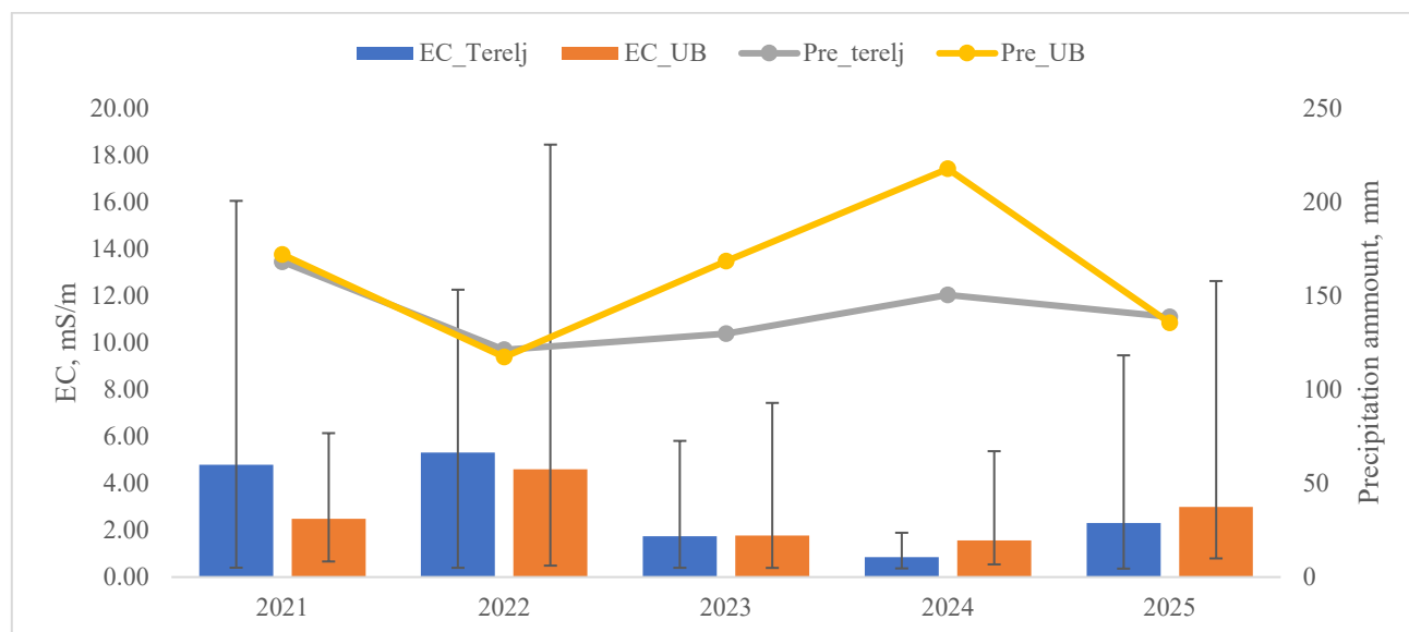
Figure 13. Arithmetic mean electrical conductivity (EC) and precipitation amount at the Ulaanbaatar and Terej sites during the May–October monitoring periods, 2021–2025. Error bars indicate the minimum and maximum measured EC values.
