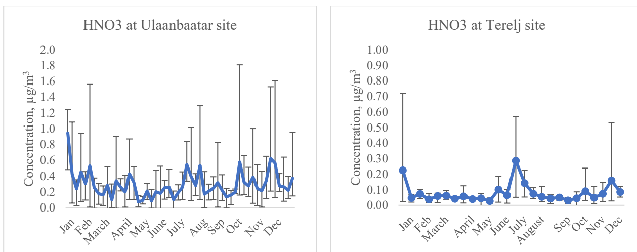
Figure 9. Nitric acid concentration at sampling sites. Error bars indicate the minimum and maximum measured concentrations during the monitoring period.
