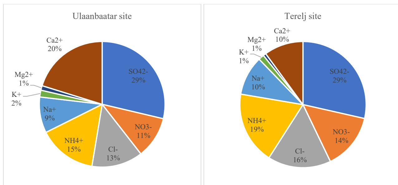
Figure 11. Relative composition of particulate major ions measured by the filter-pack method at Ulaanbaatar and Terelj, 2021–2025
