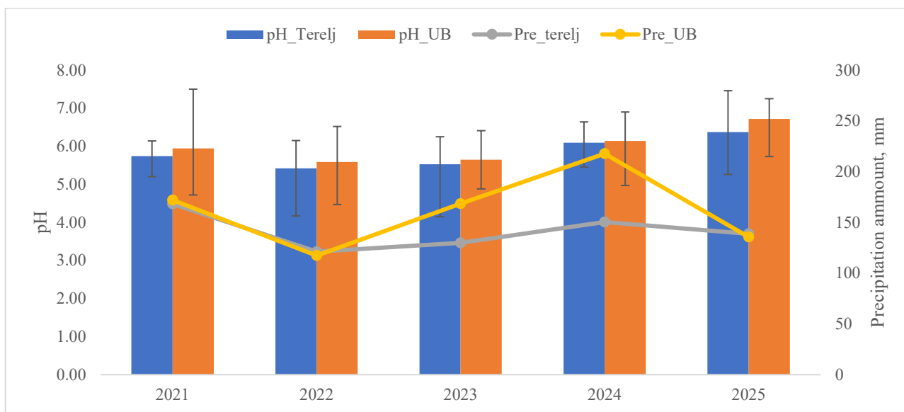
Figure 12. Arithmetic mean pH and total precipitation amount at the Ulaanbaatar and Terelj sites during the May–October monitoring periods, 2021–2025. Error bars indicate the minimum and maximum measured pH values.
