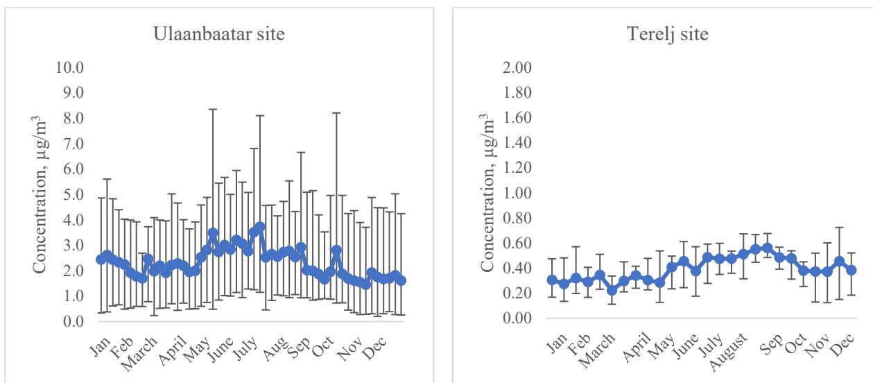
Figure 10. Hydrochloric acid concentration at sampling sites. Error bars indicate the minimum and maximum measured concentrations during the monitoring period.
