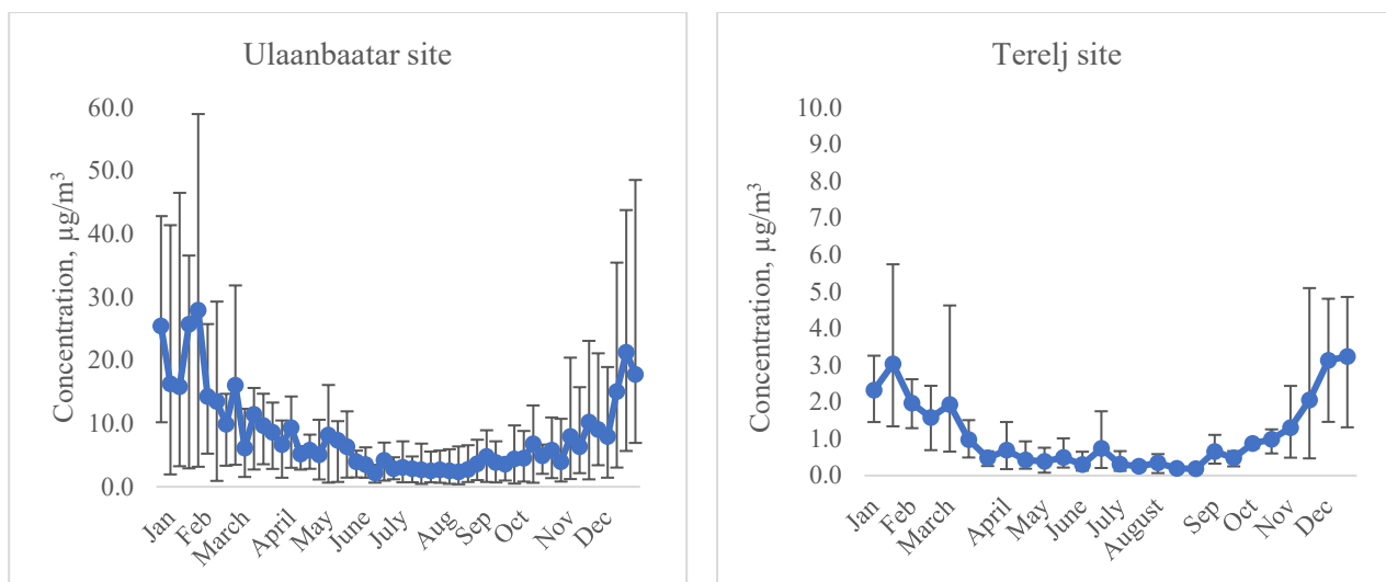
Figure 7. Sulfur dioxide concentration at sampling sites. Error bars indicate the minimum and maximum measured concentrations during the monitoring period.
