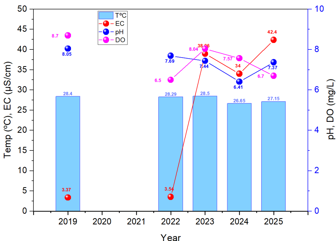
Figure 2.8. Result of annual physical parameters for inland aquatic of Nam Hum Lake
