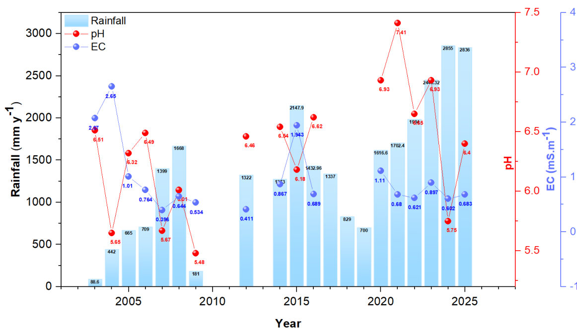
Figure 2.2. Annual variation of rainfall amount, pH and EC in Vientiane.
