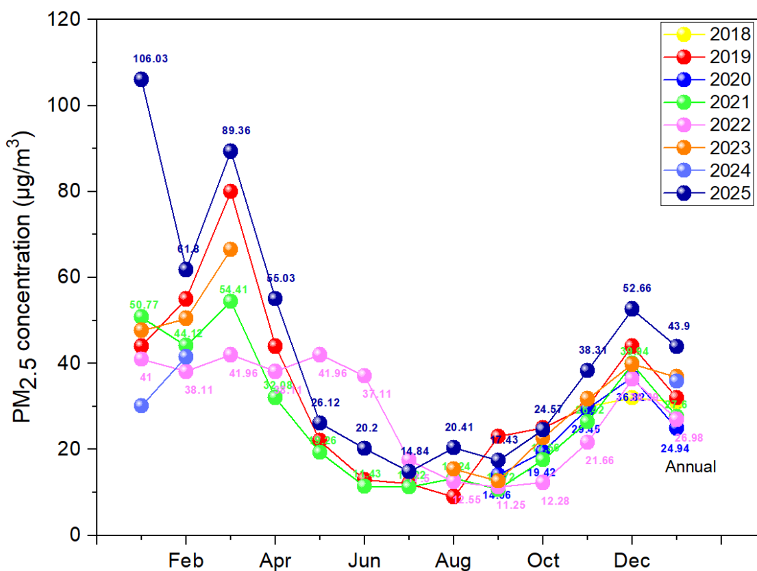
Figure 2.7. Annual variation of PM 2.5 concentration in Vientian Capital (2018 to 2025)
