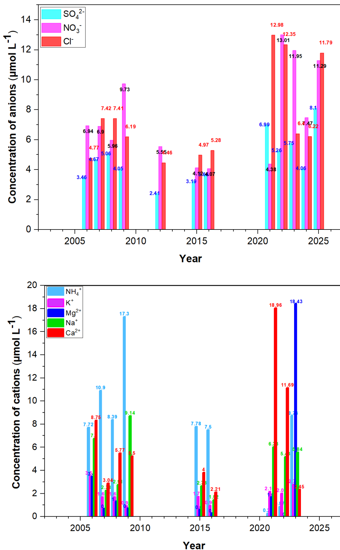
Figure 2.5. The values concentration of anions and cations during 2002 to 2025
