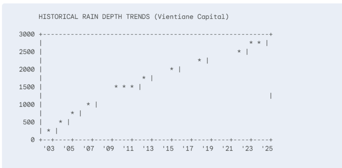
Figure 2.1. Historical rain depth trends (Vientiane Capital)
