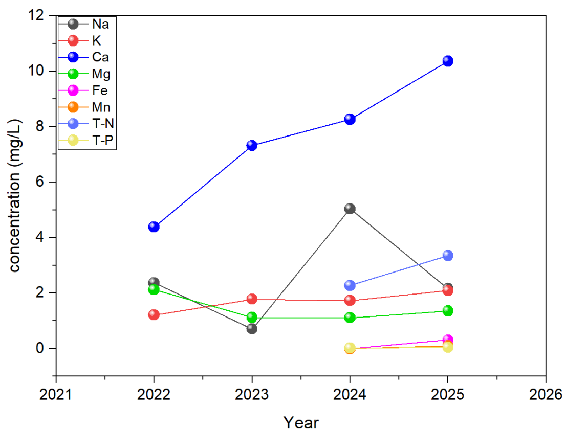
Figure 2.9. Result of annual chemical parameters for inland aquatic of Nam Hum Lake
