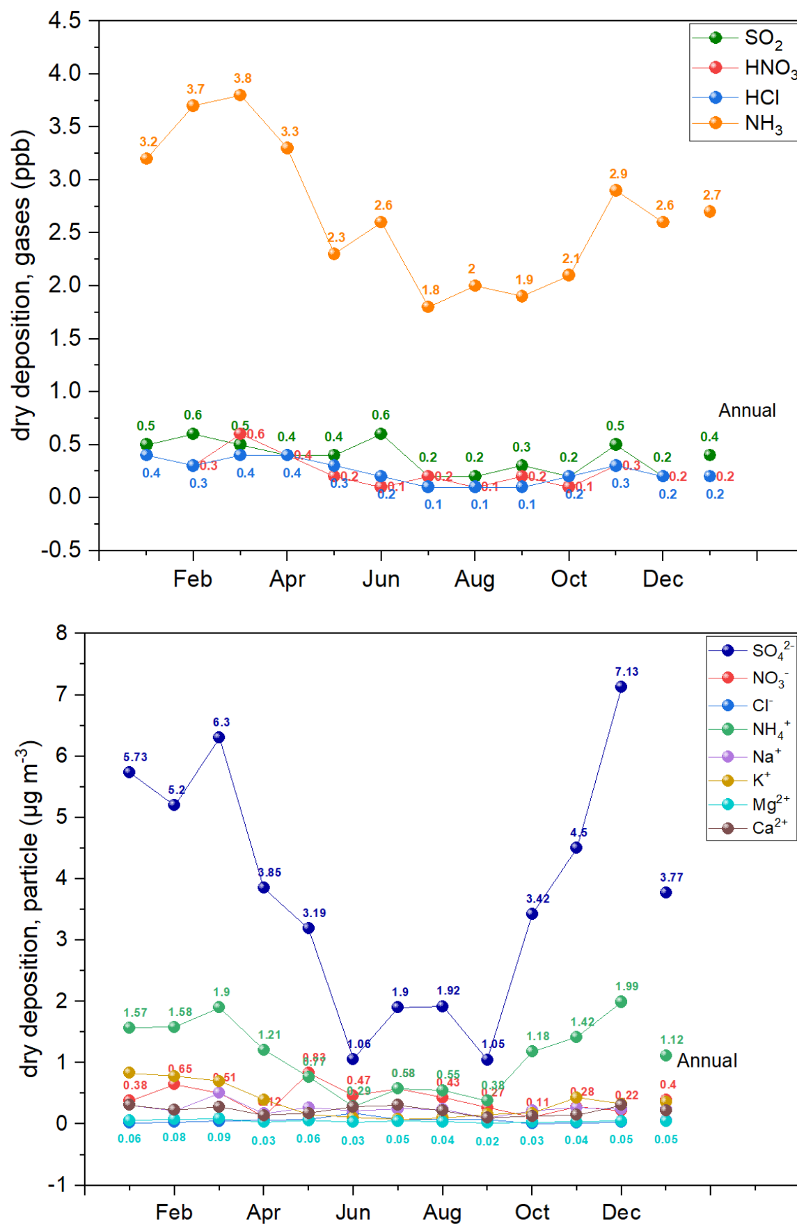
Figure 2.6. Technically seasonal atmospheric components (dry deposition) in Vientiane, 2016
