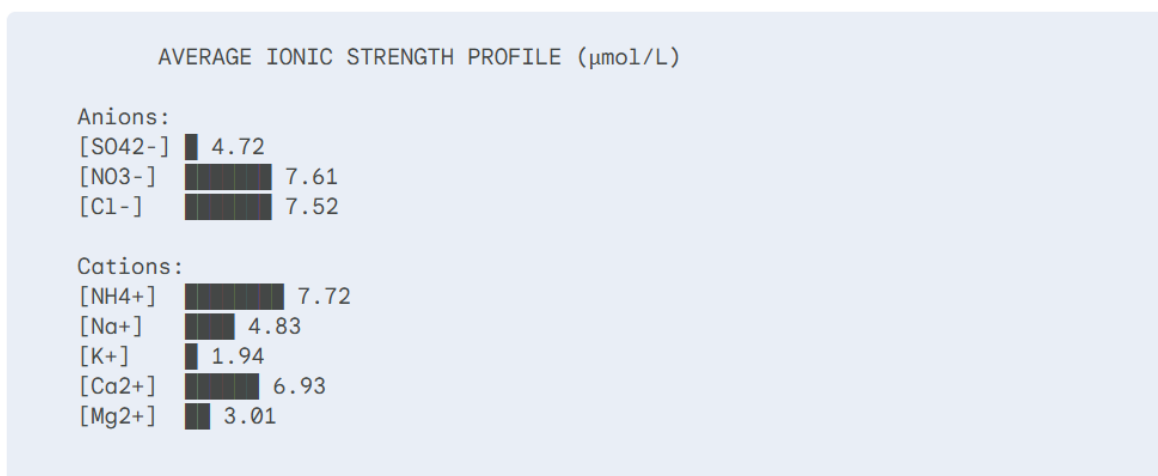
Figure 2.4. Average ionic strength profile ( \mu\text{mol/L} )
