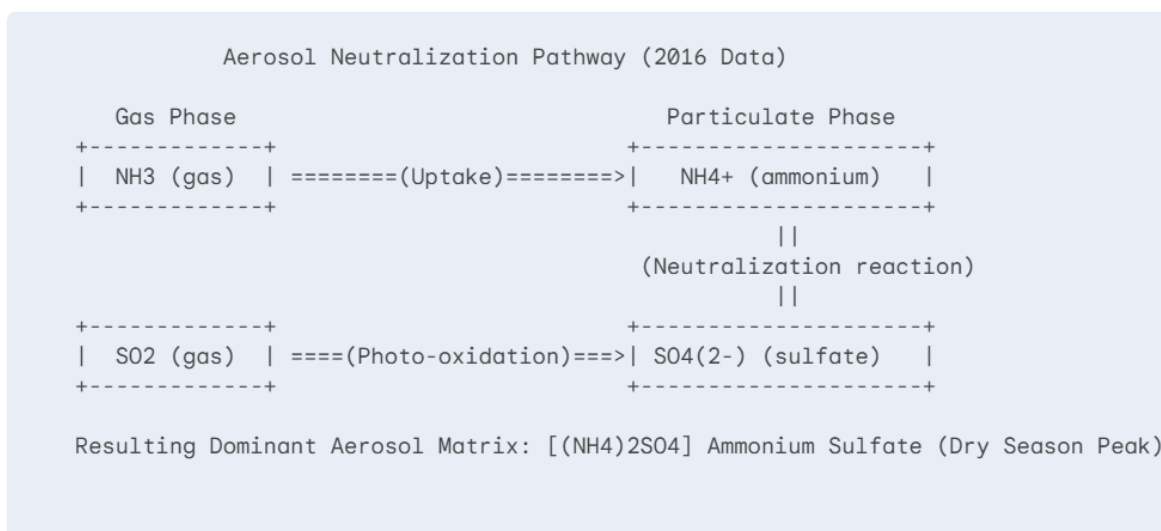
Figure 2.7. Aerosol neutralization pathway (2016 data)
