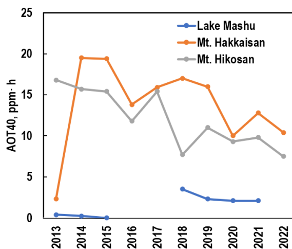
Figure 19. Changes in AOT40 at the outer rim of Lake Mashu, Mt. Hakkaisan, and Mt. Hikosan.
