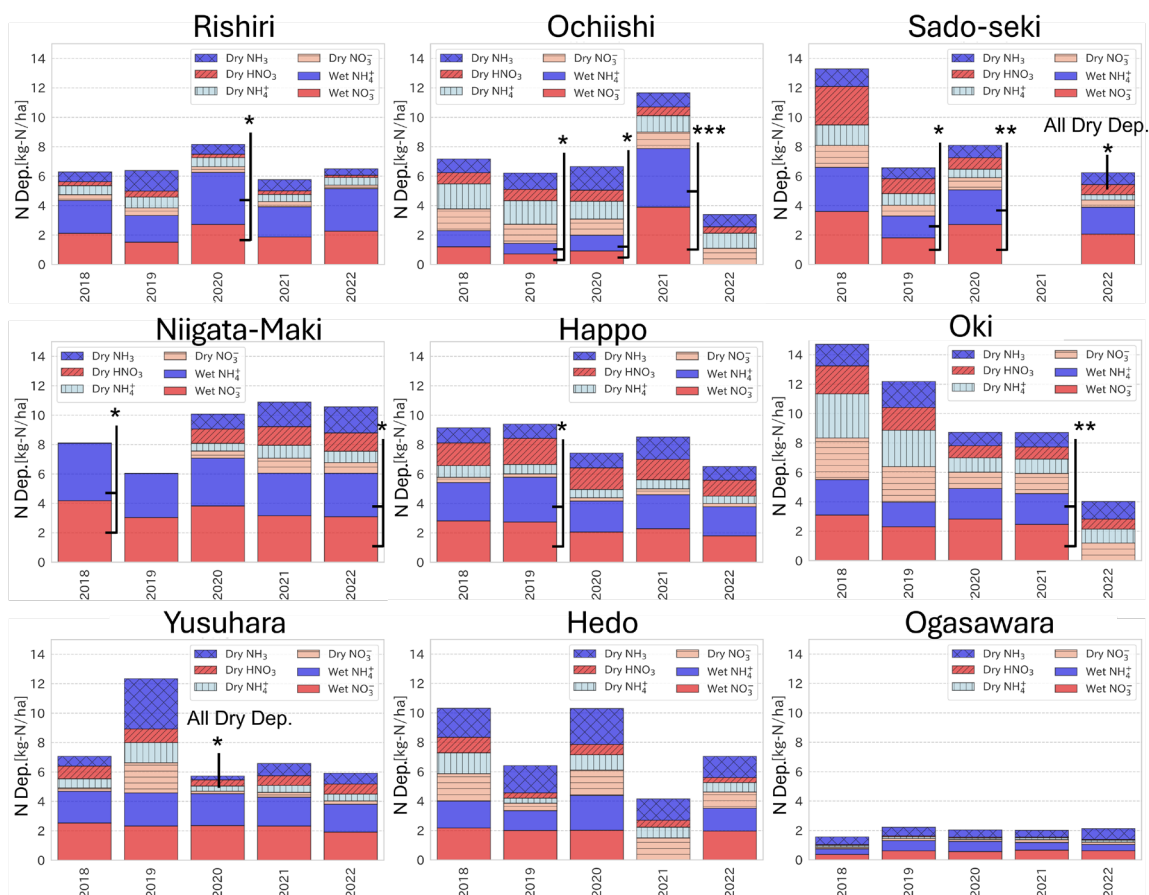
Figure 6. Annual total nitrogen deposition at each site (FY2018–FY2022)
