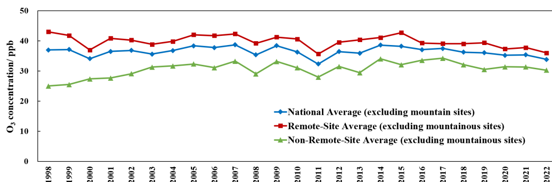
Figure 7. Long-term trends in annual mean ozone concentrations at remote and non-remote sites.
