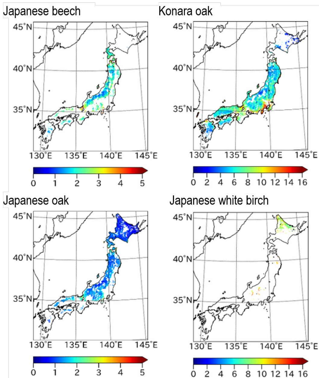
Figure 20. Mean distribution of the estimated reduction in carbon dioxide uptake due to ozone during 2015–2019 (based on simulation model results).
