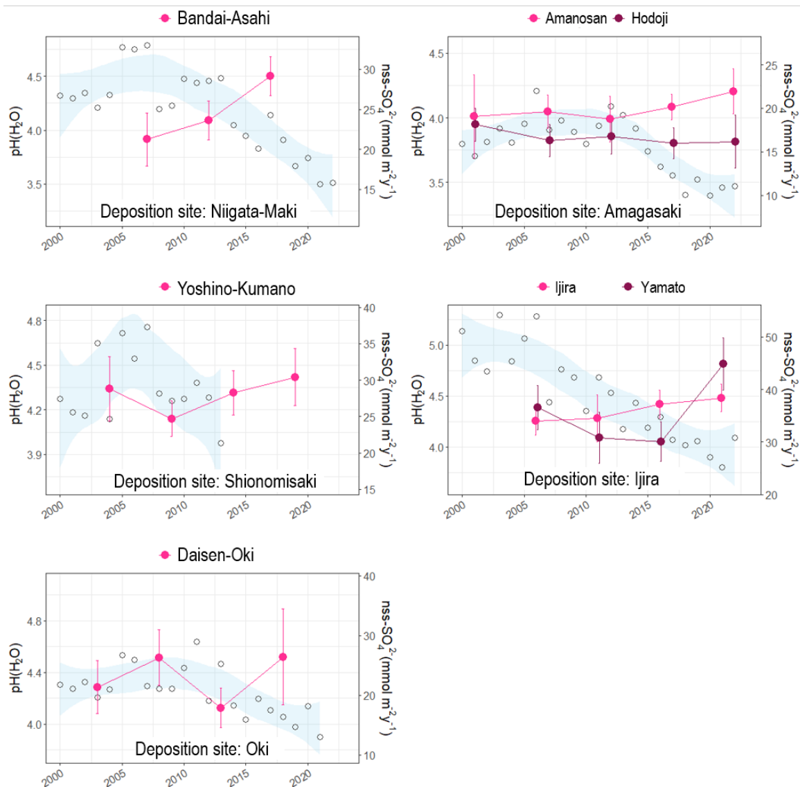
Figure 21. Long-term trends in soil pH ( \text{H}_2\text{O} ) and wet deposition of \text{nss-SO}_4^{2-} .
