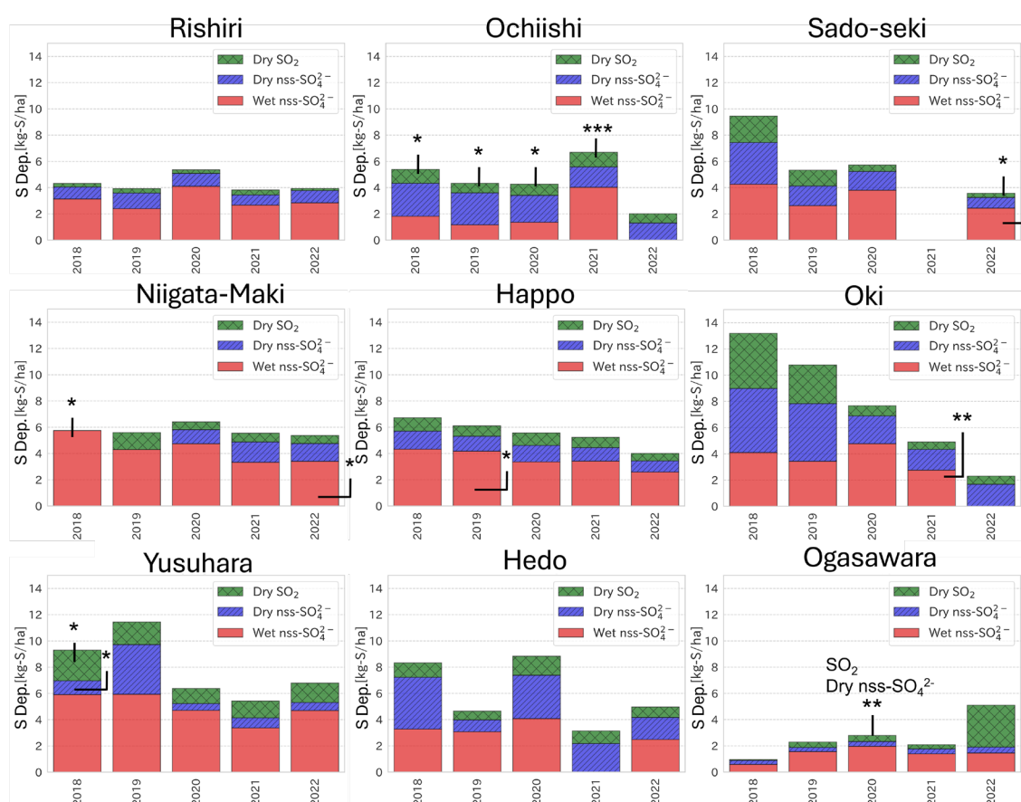
Figure 5. Annual total sulfur deposition at each site (FY2018–FY2022)
