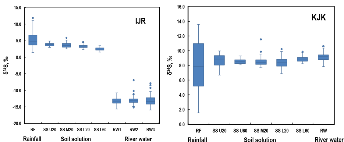
Figure 18. Vertical changes in sulfur isotope ratios ( \delta^{34}\text{S} ) from precipitation (RF), through soil solution (SS), to stream water (RW) in the Ijira Lake catchment (IJR; left) and the Kajikawa catchment (KJK; right).
