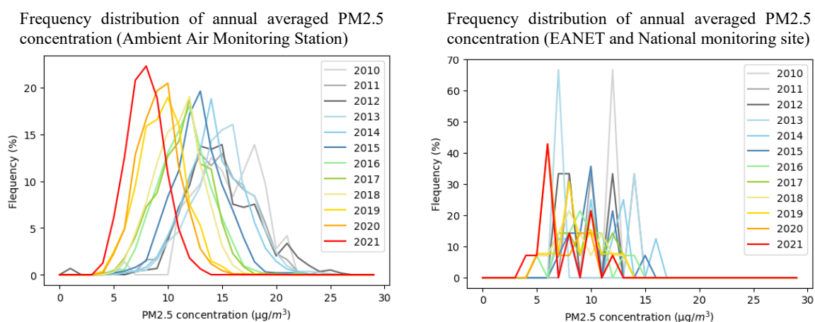
Figure 11. Relative frequency distribution of annual mean PM 2.5 concentrations (FY2010–FY2021). (Left) Ambient air monitoring stations; (Right) EANET and national monitoring stations.
