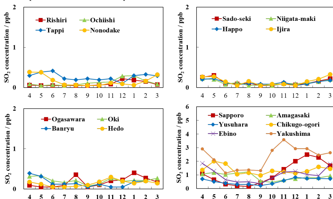
Figure 12. Monthly variation in SO 2 concentration (average for FY2018–FY2022).
