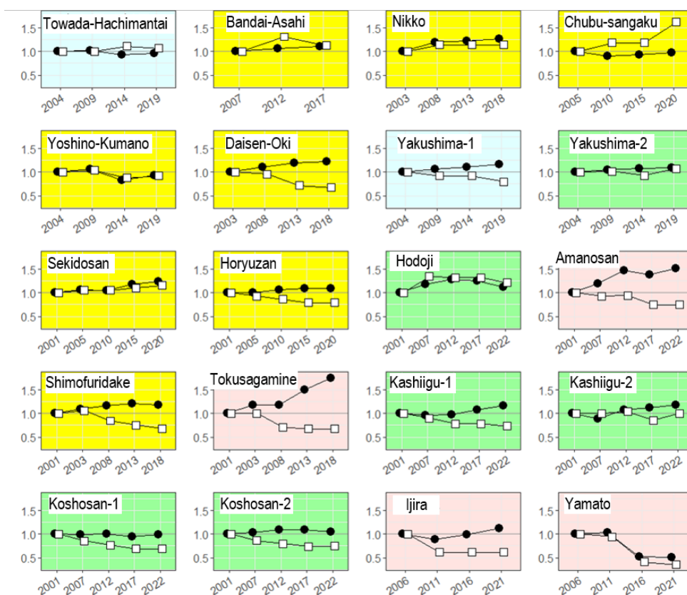
Figure 15. Long-term trends in total basal area and tree density.
