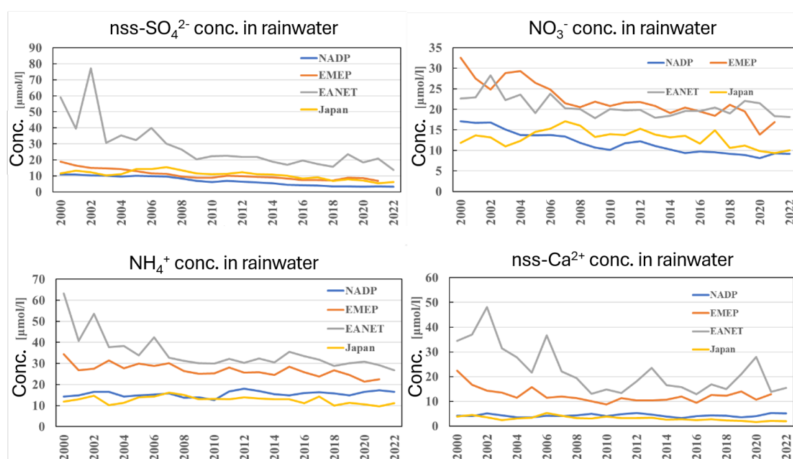
Figure 2-2. Comparison of trends in concentrations of chemical constituents in precipitation between Japan and other international monitoring networks (nss-SO 4 2- : Non-sea salt sulfate ion, NO 3 - : Nitrate ion, NH 4 + : Ammonium ion, and nss-Ca 2+ : Non-sea salt calcium ion).
