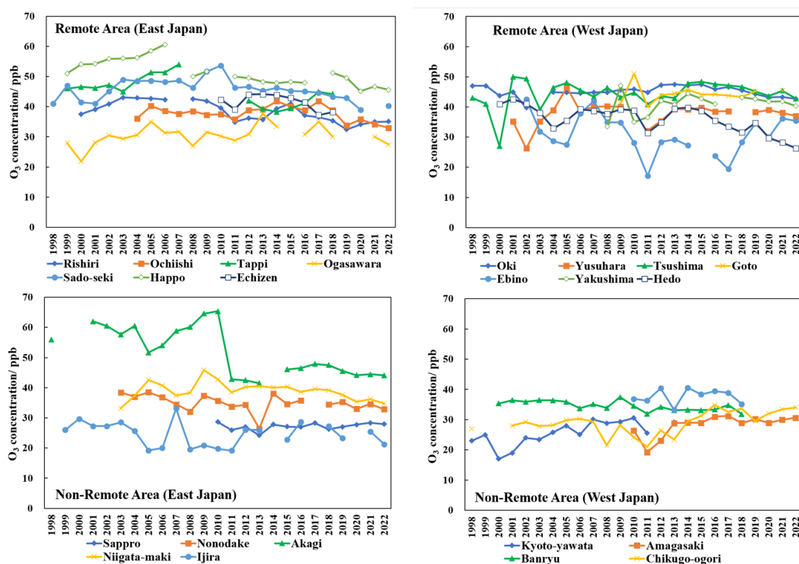
Figure 8. Long-term trends in ozone concentrations at individual sites.
