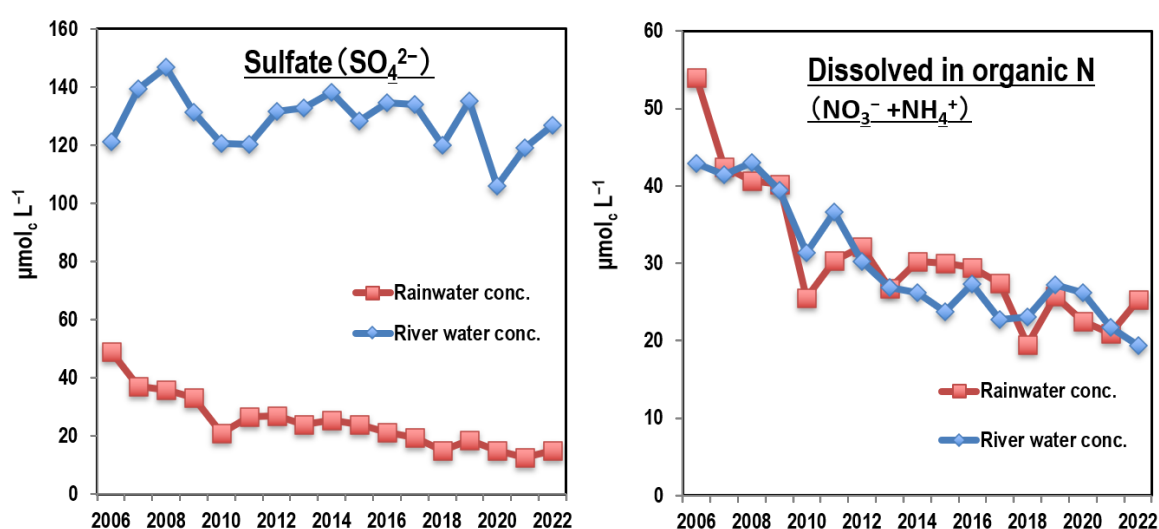
Figure 16. Long-term trends in volume-weighted mean concentrations of \text{SO}_4^{2-} and DIN in the Ijira Lake catchment.
