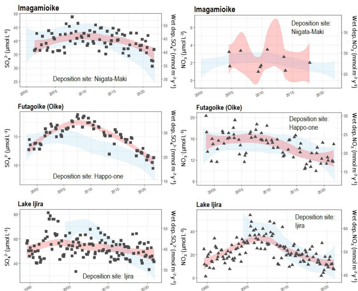
Figure 22. Changes in \text{SO}_4^{2-} concentrations (left) and \text{NO}_3^- concentrations (right) in inland water associated with long-term changes in wet deposition.
