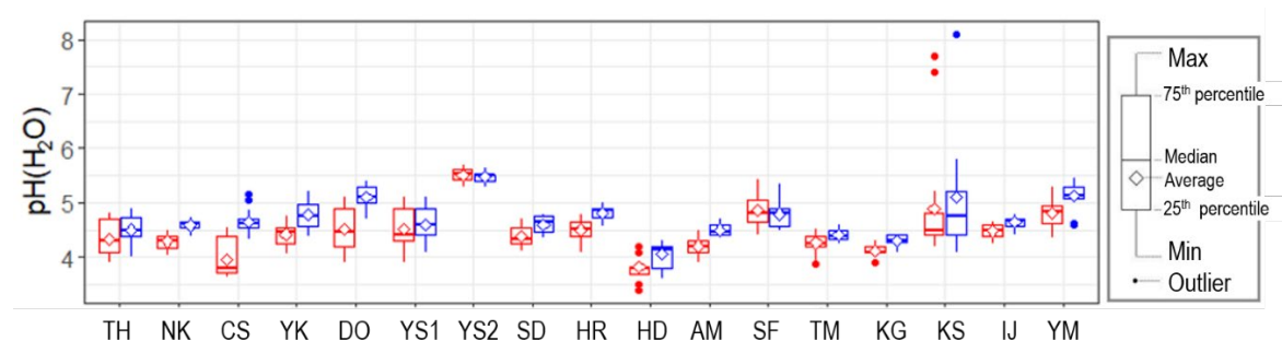
Figure 14. Range of soil pH (H 2 O) values (FY2018–FY2022 survey).
