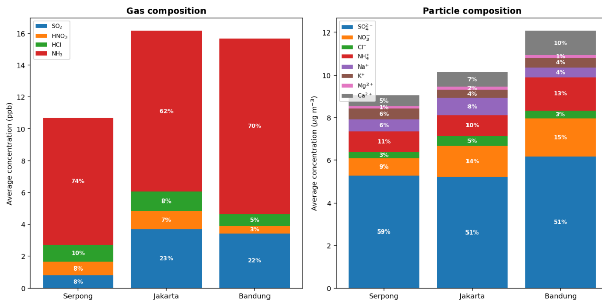
Figure 11. Gas and particle composition in Serpong, Jakarta and Bandung from 2020 – 2022
