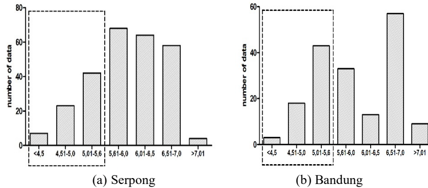
Figure 6. pH distribution in Serpong and Bandung during 2020-2022 Sampling periode: event (data source: EMC and BRIN)
