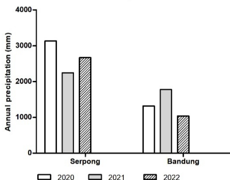
Figure 4. Annual precipitation in 2020-2022
