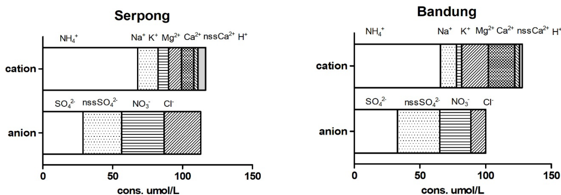
Figure 10. Chemical composition of rainwater in Serpong and Bandung during 2020-2022
