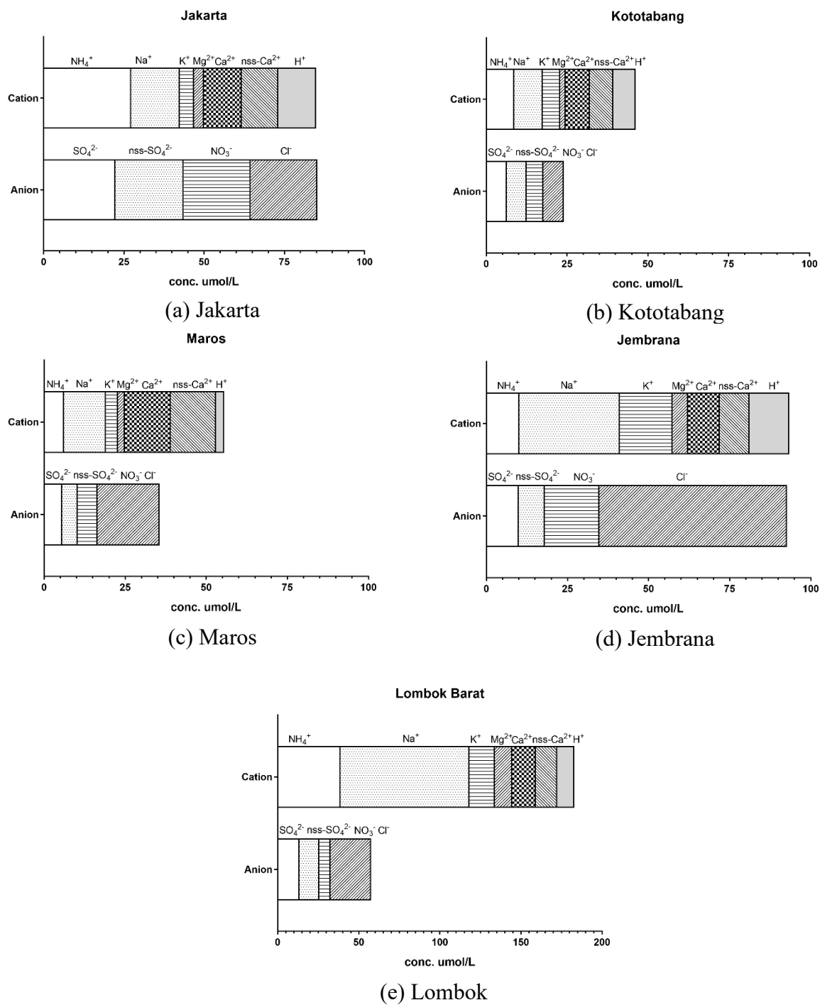
Figure 9. Chemical composition of rainwater in Jakarta, Kototabang, Maros, Jembrana and Lombok during 2020-2024
