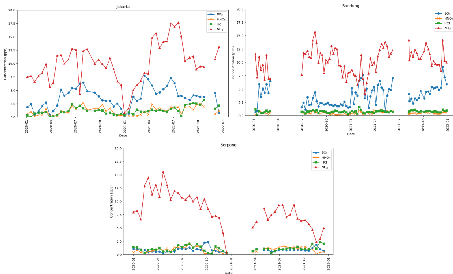
Figure 12. Trend of Gas Composition in Serpong, Jakarta, and Bandung from 2020 - 2022
