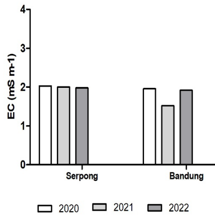
Figure 8. Annual average of EC in Serpong and Bandung during 2020-2022
