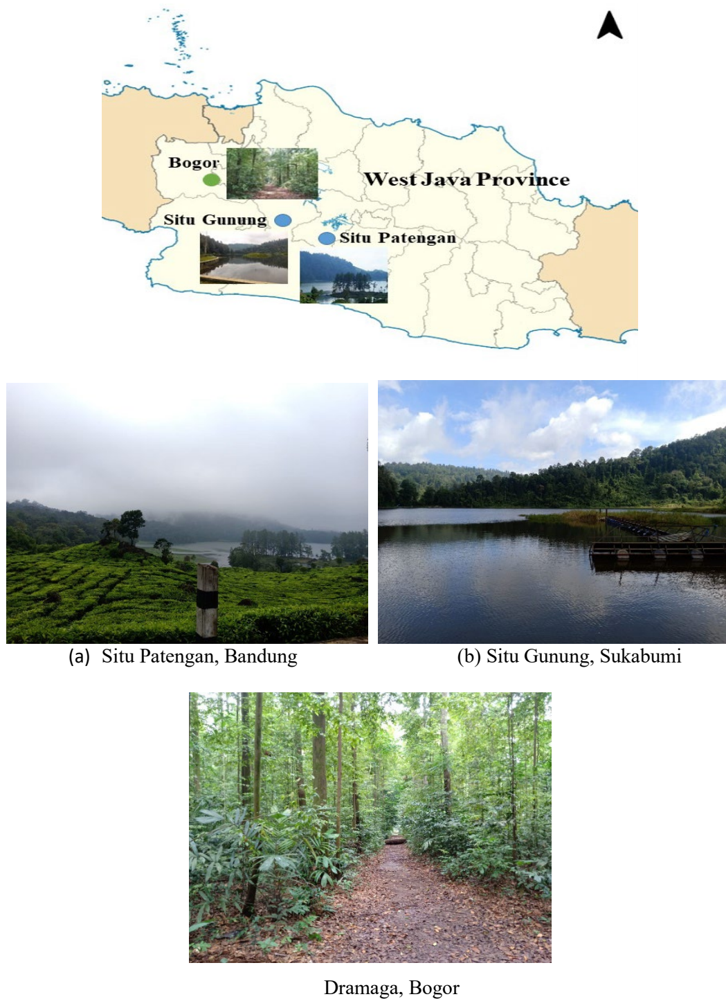
Figure 2. Ecological impact sites
