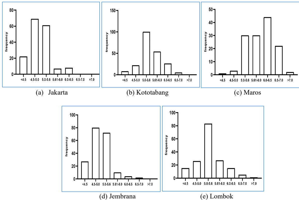
Figure 5. pH distribution in Jakarta, Kototabang, Maros, Jembrana and Lombok during 2020-2024 Sampling periode: biweekly (data source: BMKG Jakarta)
