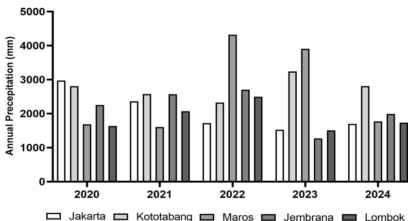
Figure 3. Annual precipitation of BMKG's sites in 2020-2024
