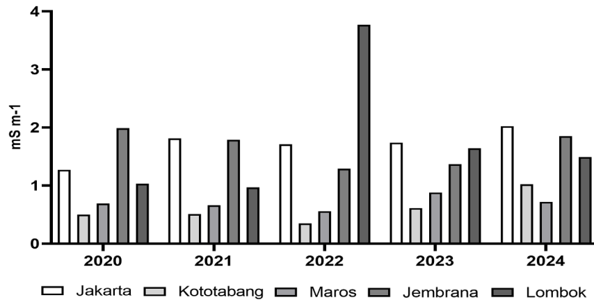
Figure 7. Annual average of EC in Jakarta, Kototabang, Maros, Jembrana and Lombok during 2020-2024
