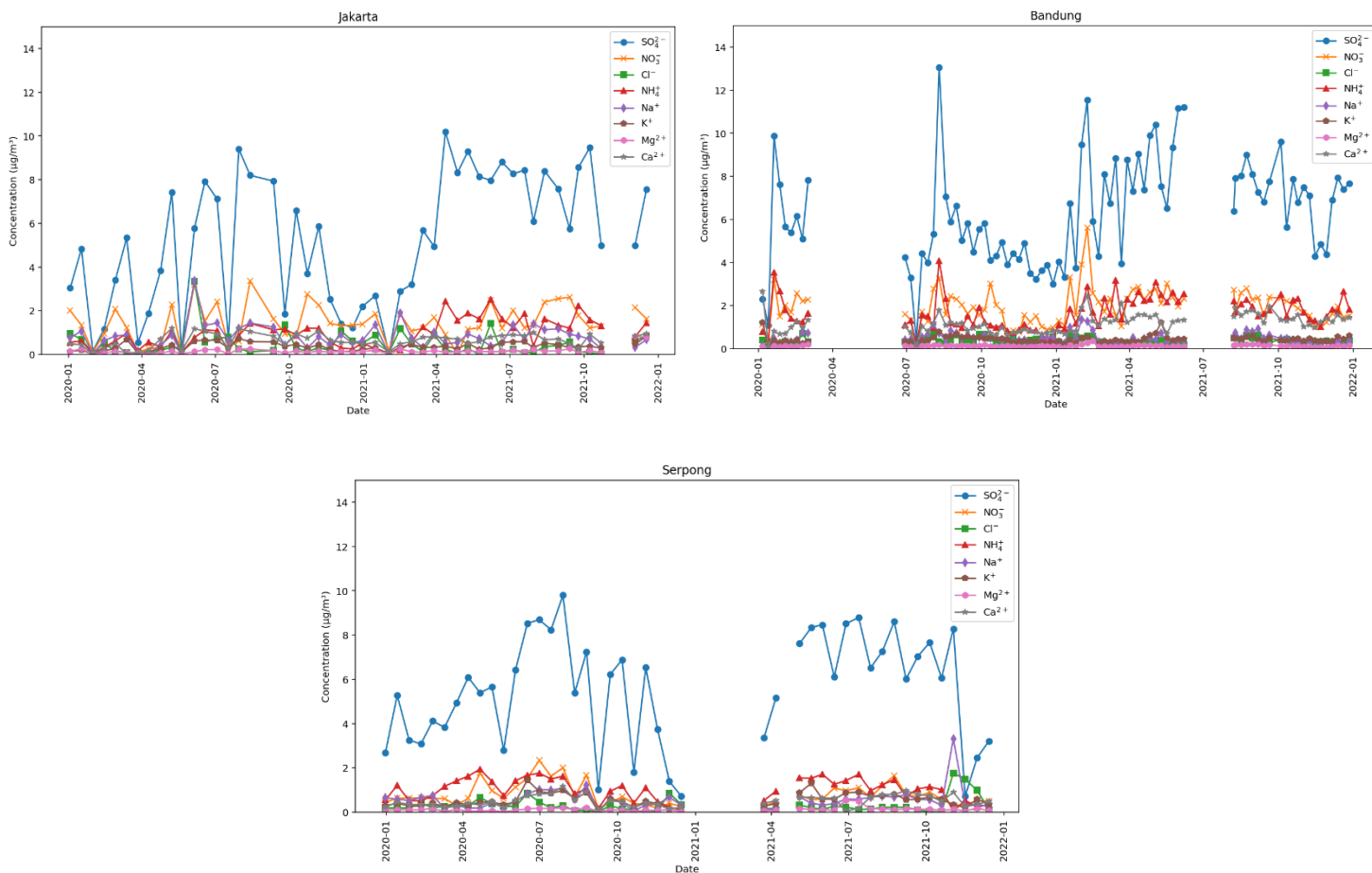
Figure 13. Trend of Particle Composition in Serpong, Jakarta and Bandung from 2020 - 2022
